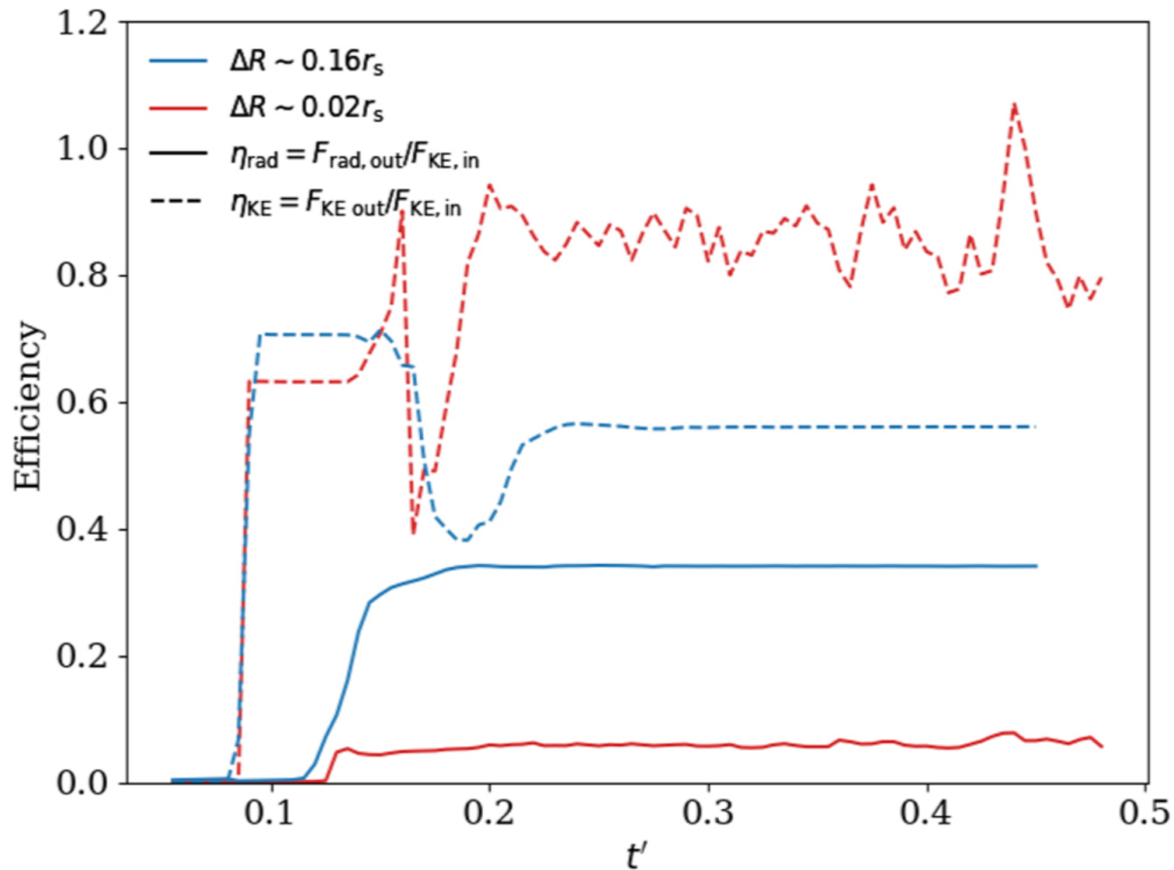
Figure 4. from Xiaoshan Huang et al 2023 Astrophys. J. 953 doi:10.3847/1538-4357/ace0be https://dx.doi.org/10.3847/1538-4357/ace0be © 2023. The Author(s). Published by the American Astronomical Society.
