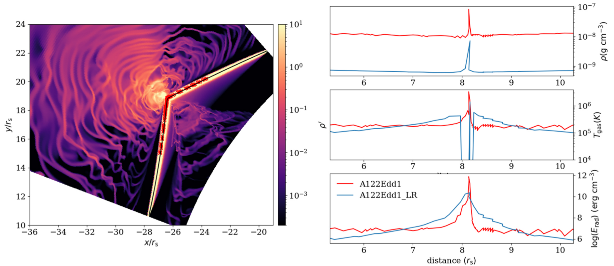
Figure 22. from Xiaoshan Huang et al 2023 Astrophys. J. 953 doi:10.3847/1538-4357/ace0be https://dx.doi.org/10.3847/1538-4357/ace0be © 2023. The Author(s). Published by the American Astronomical Society.
