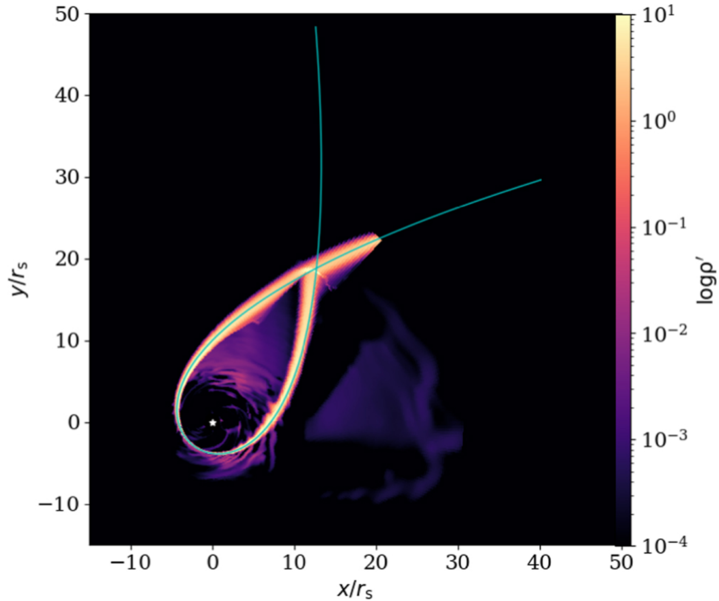
Figure 21. from Xiaoshan Huang et al 2023 Astrophys. J. 953 doi:10.3847/1538-4357/ace0be https://dx.doi.org/10.3847/1538-4357/ace0be © 2023. The Author(s). Published by the American Astronomical Society.
