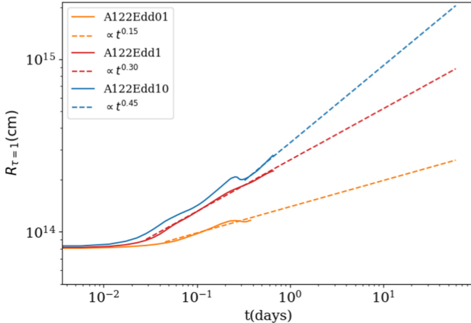
Figure 17. from Xiaoshan Huang et al 2023 Astrophys. J. 953 doi:10.3847/1538-4357/ace0be https://dx.doi.org/10.3847/1538-4357/ace0be © 2023. The Author(s). Published by the American Astronomical Society.
