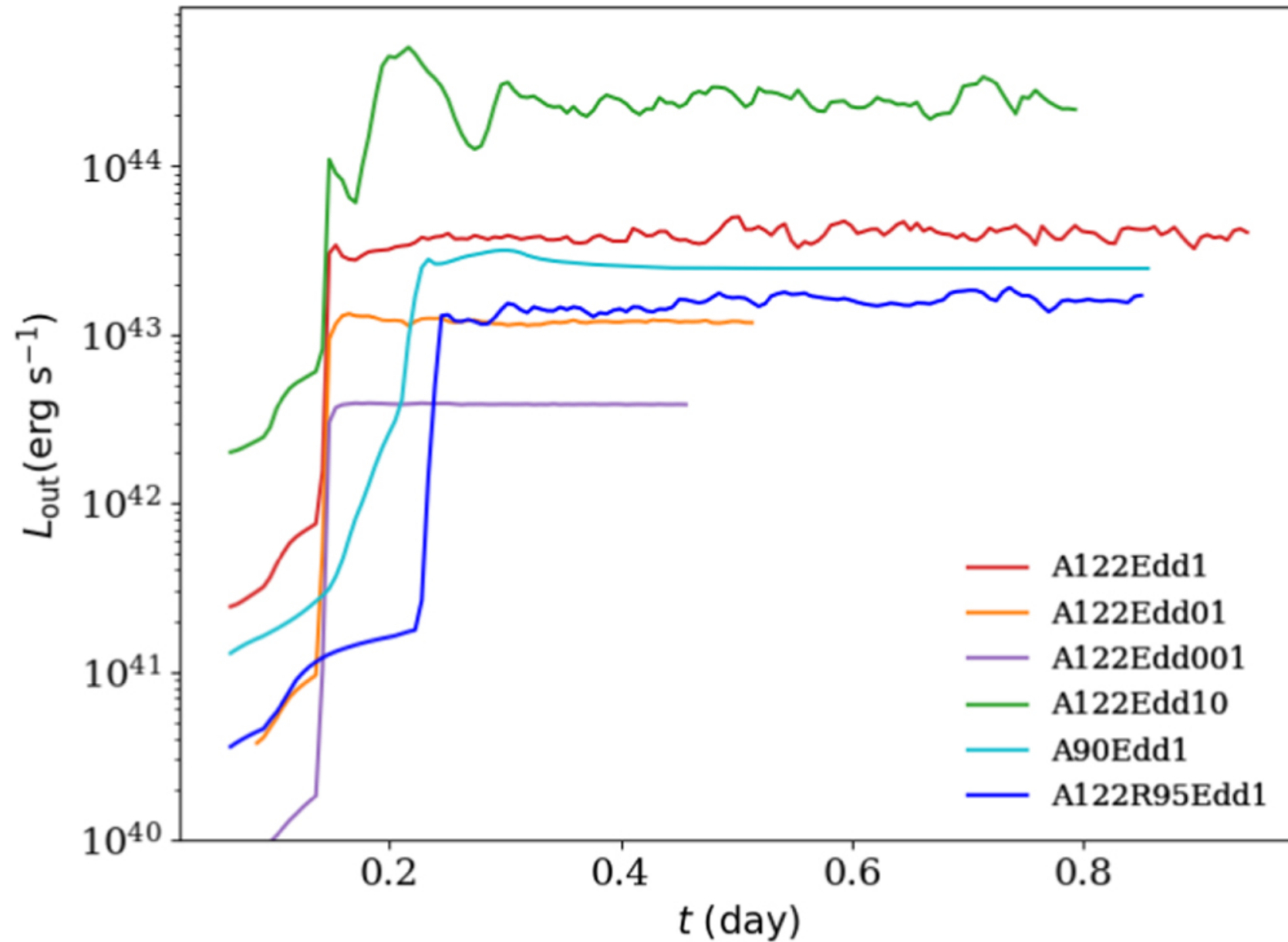
Figure 15. from Xiaoshan Huang et al 2023 Astrophys. J. 953 doi:10.3847/1538-4357/ace0be https://dx.doi.org/10.3847/1538-4357/ace0be © 2023. The Author(s). Published by the American Astronomical Society.
