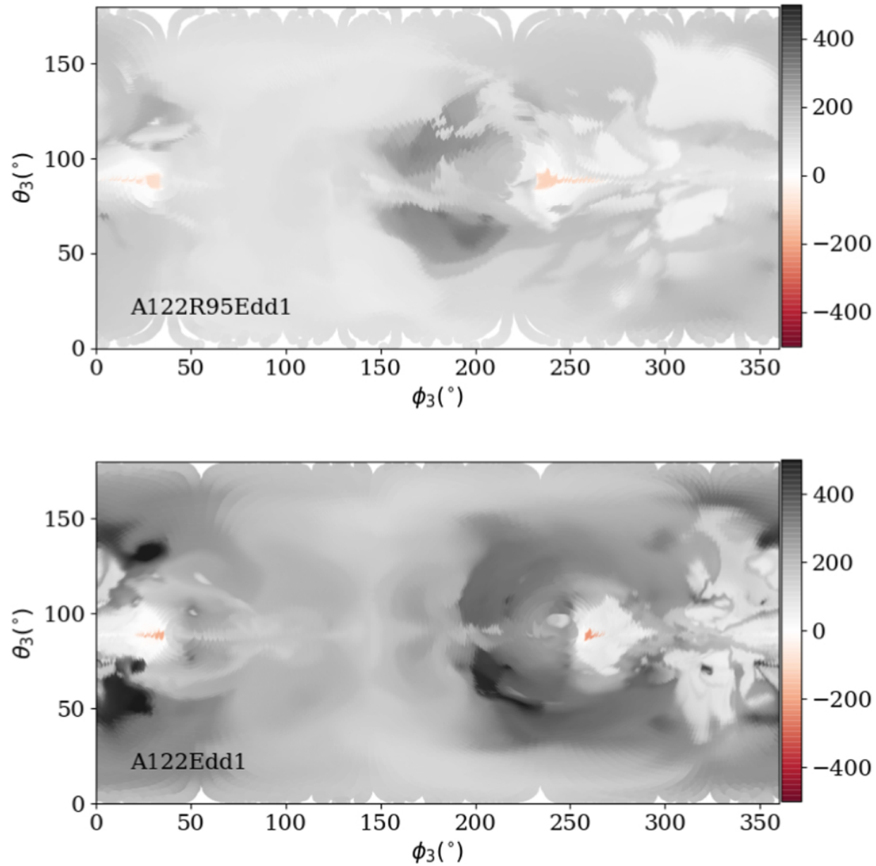
Figure 14. from Xiaoshan Huang et al 2023 Astrophys. J. 953 doi:10.3847/1538-4357/ace0be https://dx.doi.org/10.3847/1538-4357/ace0be © 2023. The Author(s). Published by the American Astronomical Society.
