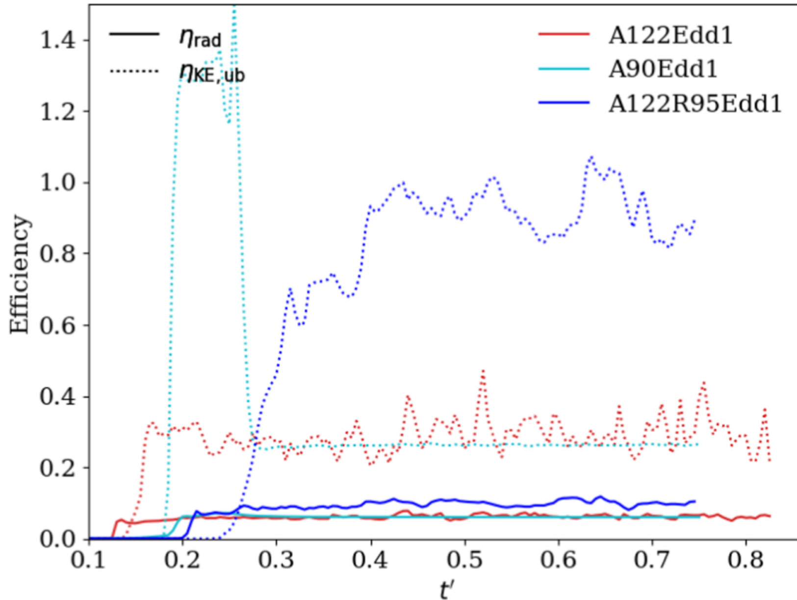
Figure 12. from Xiaoshan Huang et al 2023 Astrophys. J. 953 doi:10.3847/1538-4357/ace0be https://dx.doi.org/10.3847/1538-4357/ace0be © 2023. The Author(s). Published by the American Astronomical Society.
