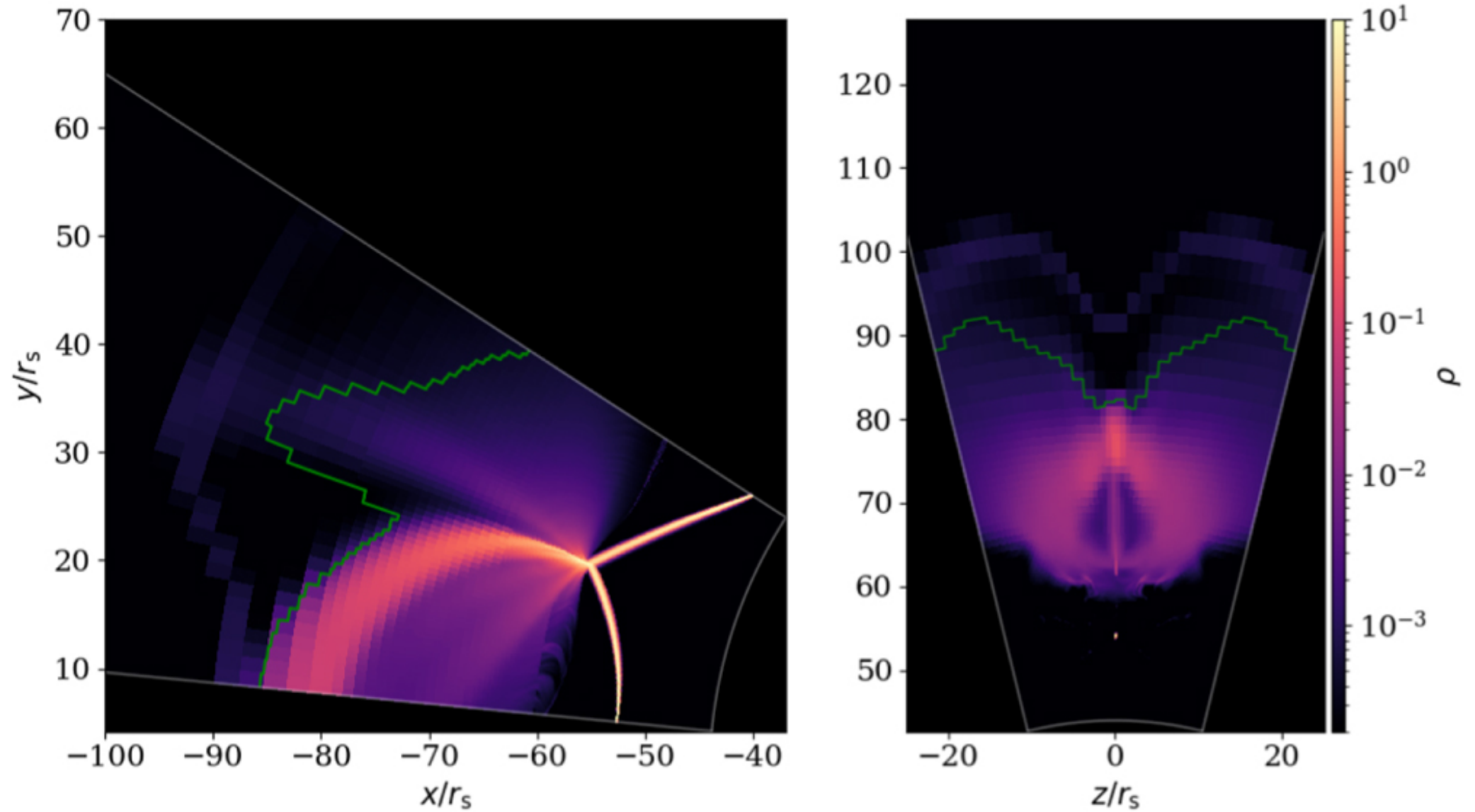
Figure 11. from Xiaoshan Huang et al 2023 Astrophys. J. 953 doi:10.3847/1538-4357/ace0be https://dx.doi.org/10.3847/1538-4357/ace0be © 2023. The Author(s). Published by the American Astronomical Society.
