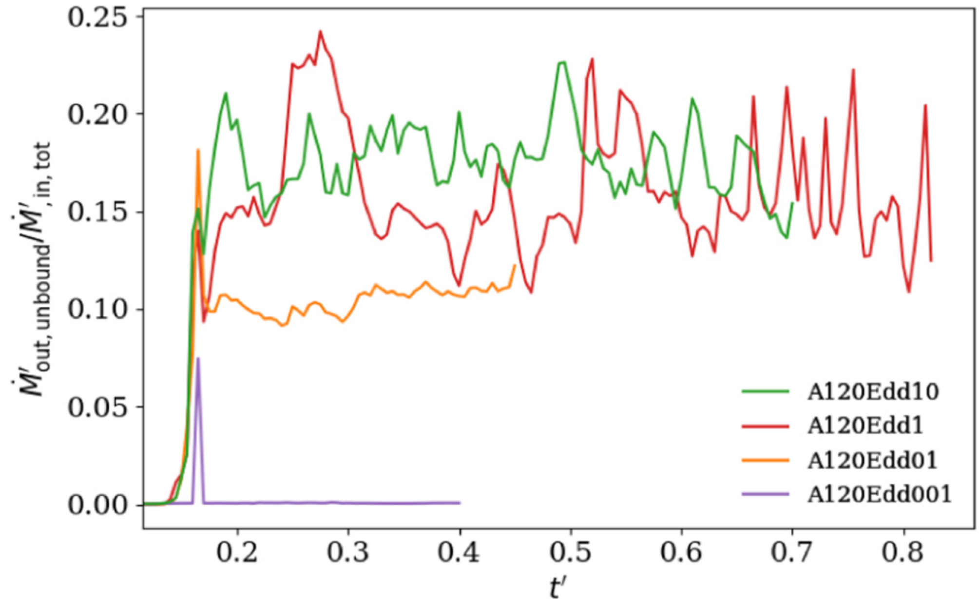
Figure 10. from Xiaoshan Huang et al 2023 Astrophys. J. 953 doi:10.3847/1538-4357/ace0be https://dx.doi.org/10.3847/1538-4357/ace0be © 2023. The Author(s). Published by the American Astronomical Society.
