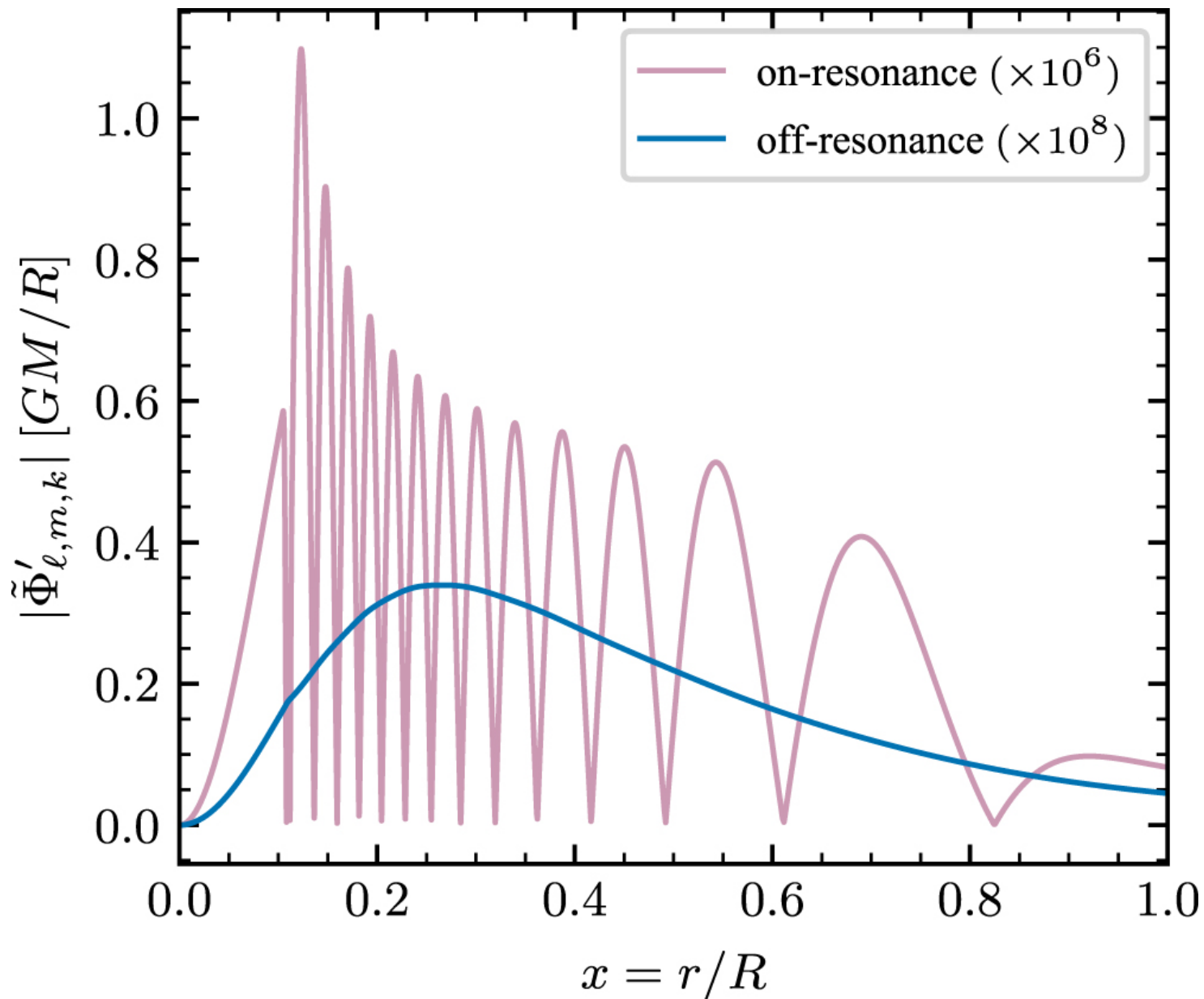
Figure 4. from R. H. D. Townsend et al 2023 Astrophys. J. 953 doi:10.3847/1538-4357/acdd5a https://dx.doi.org/10.3847/1538-4357/acdd5a © 2023. The Author(s). Published by the American Astronomical Society.
