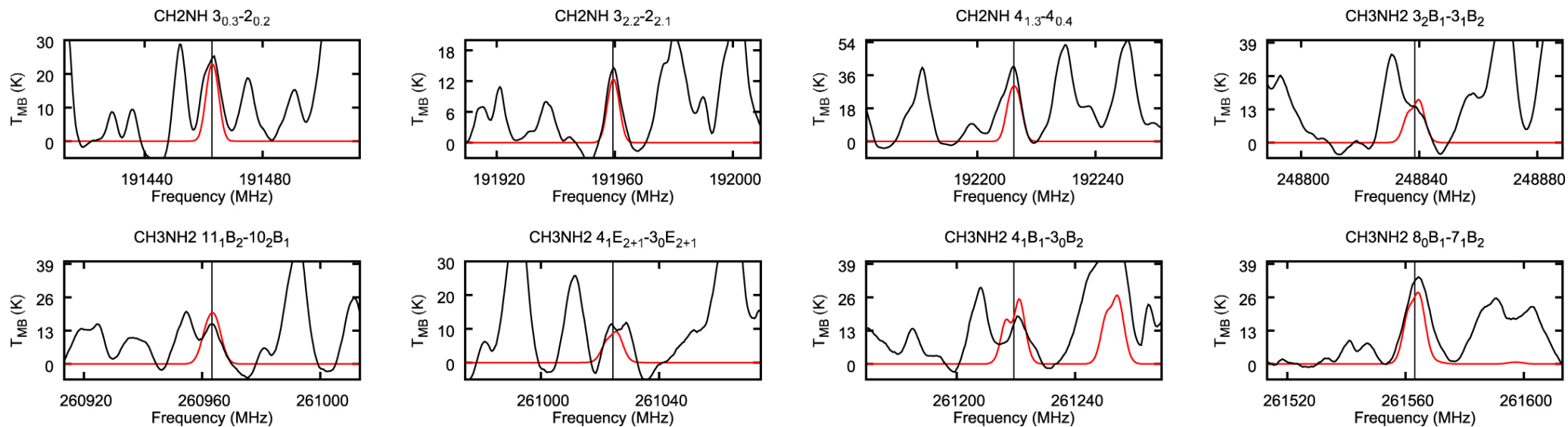
Figure 9. from Taiki Suzuki et al 2023 Astrophys. J. 954 doi:10.3847/1538-4357/acdb6d https://dx.doi.org/10.3847/1538-4357/acdb6d © 2023. The Author(s). Published by the American Astronomical Society.
