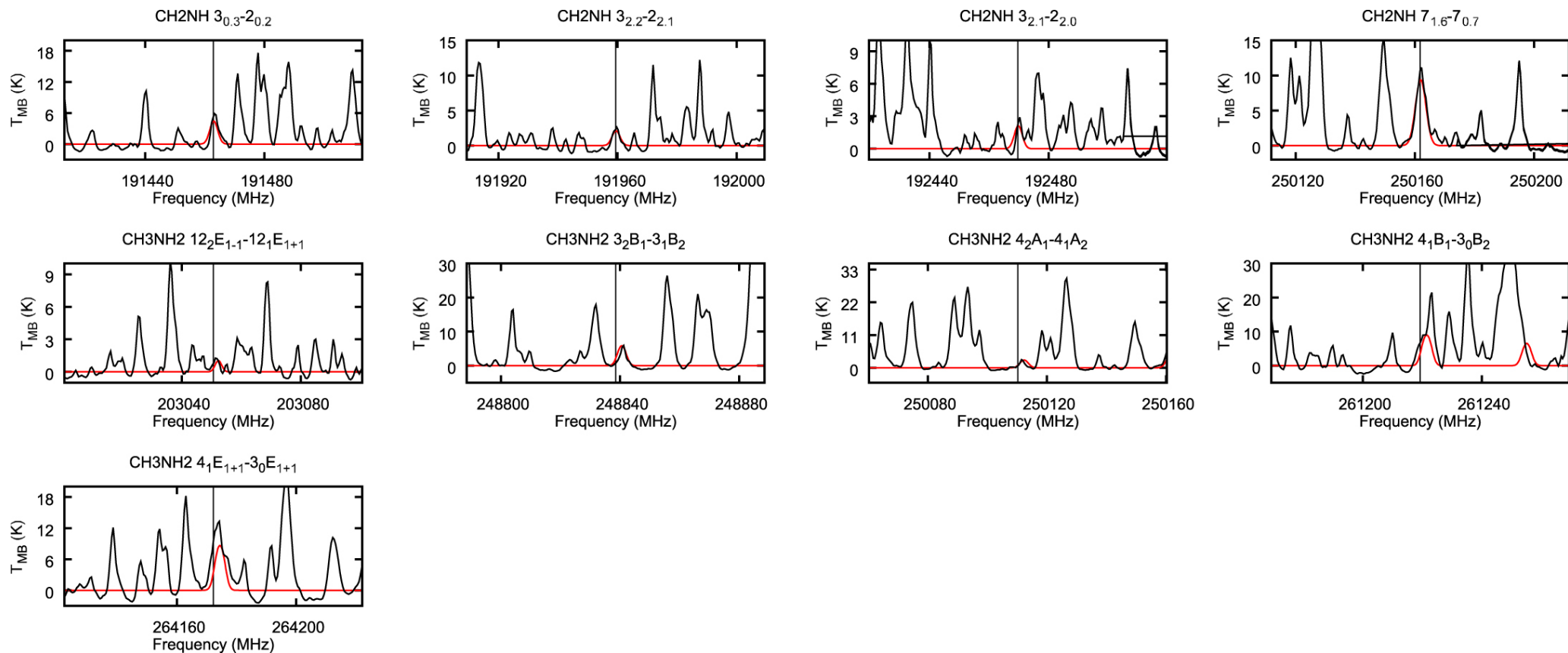
Figure 8. from Taiki Suzuki et al 2023 Astrophys. J. 954 doi:10.3847/1538-4357/acdb6d https://dx.doi.org/10.3847/1538-4357/acdb6d © 2023. The Author(s). Published by the American Astronomical Society.
