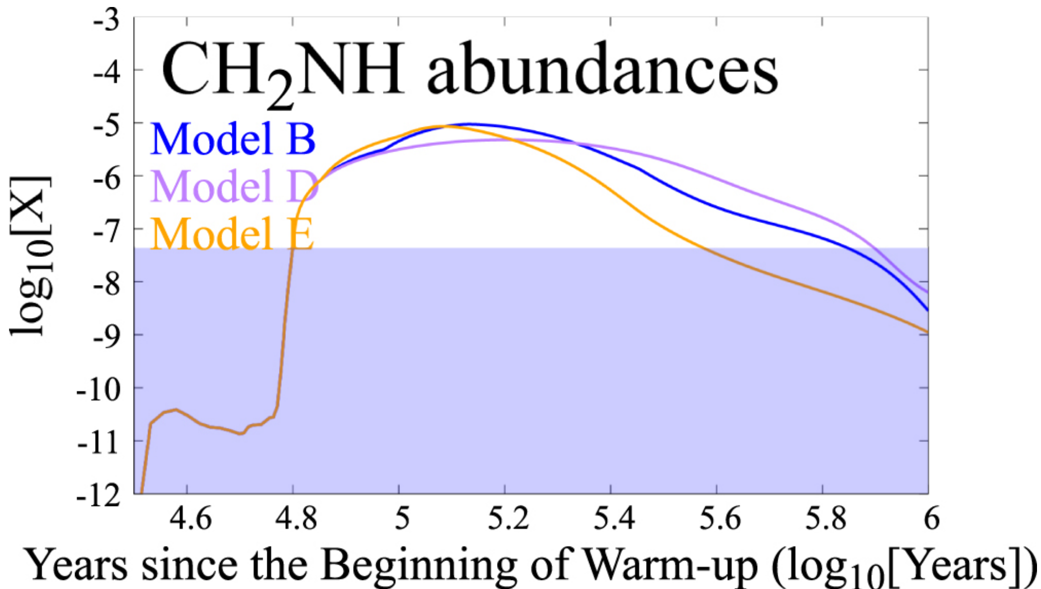
Figure 16. from Taiki Suzuki et al 2023 Astrophys. J. 954 doi:10.3847/1538-4357/acdb6d https://dx.doi.org/10.3847/1538-4357/acdb6d © 2023. The Author(s). Published by the American Astronomical Society.
