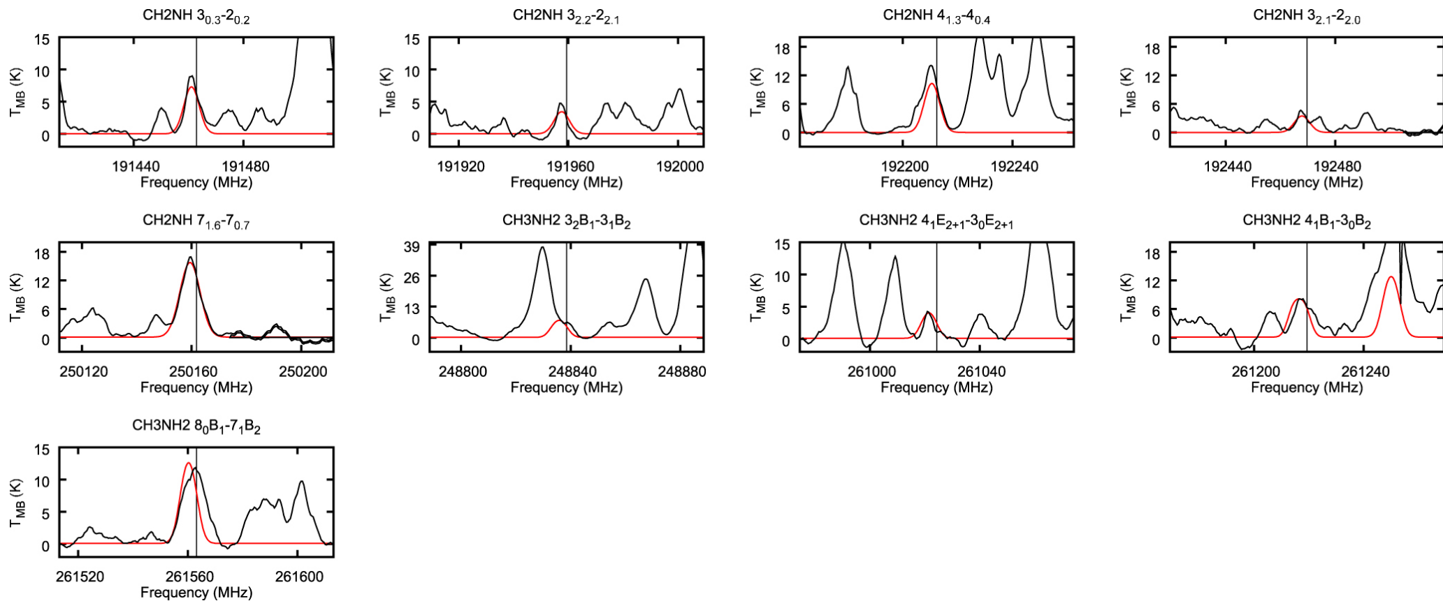
Figure 12. from Taiki Suzuki et al 2023 Astrophys. J. 954 doi:10.3847/1538-4357/acdb6d https://dx.doi.org/10.3847/1538-4357/acdb6d © 2023. The Author(s). Published by the American Astronomical Society.
