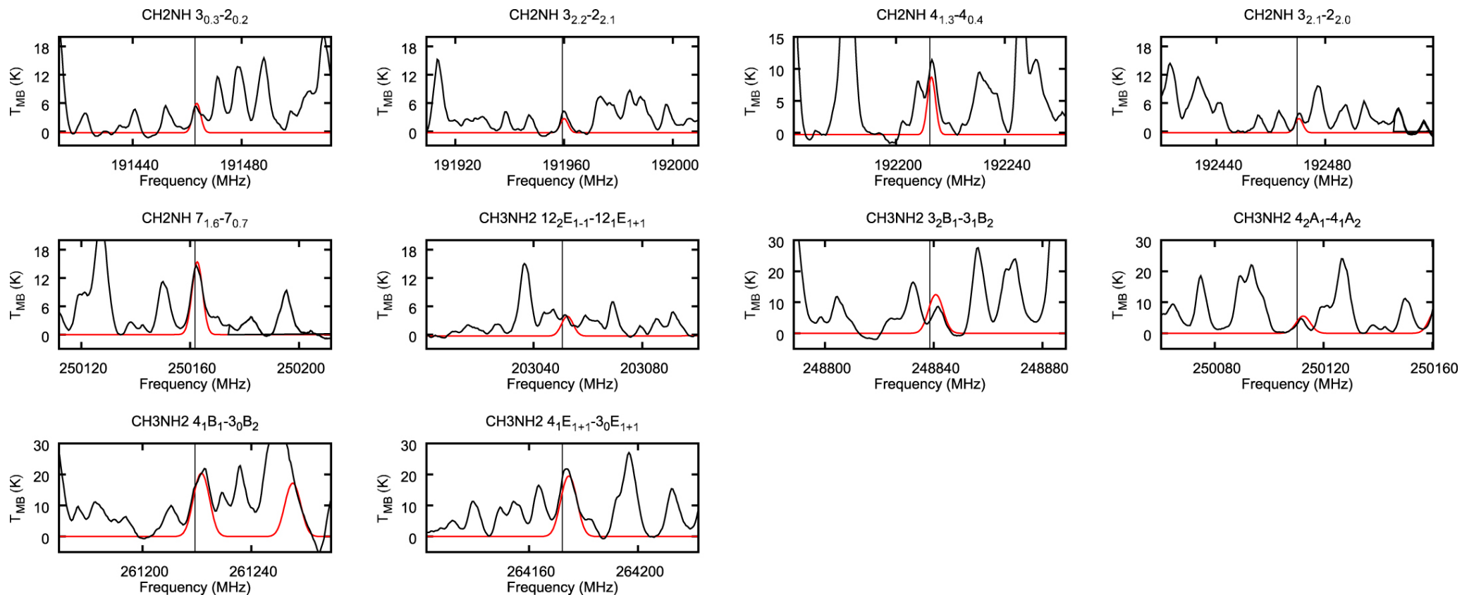
Figure 11. from Taiki Suzuki et al 2023 Astrophys. J. 954 doi:10.3847/1538-4357/acdb6d https://dx.doi.org/10.3847/1538-4357/acdb6d © 2023. The Author(s). Published by the American Astronomical Society.
