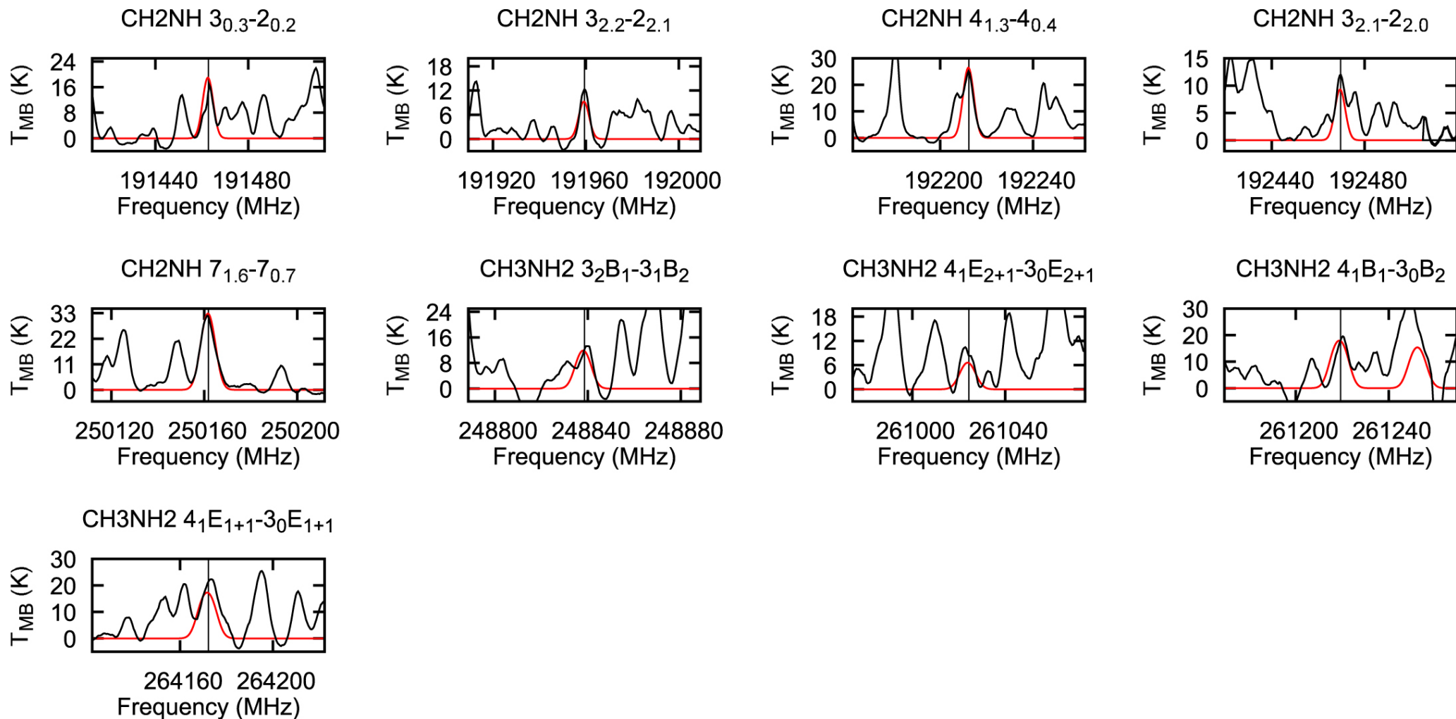
Figure 10. from Taiki Suzuki et al 2023 Astrophys. J. 954 doi:10.3847/1538-4357/acdb6d https://dx.doi.org/10.3847/1538-4357/acdb6d © 2023. The Author(s). Published by the American Astronomical Society.
