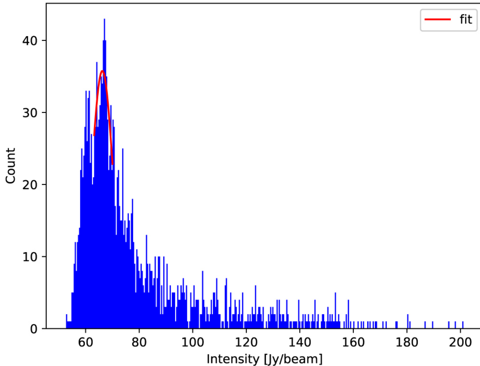
Figure 1. from Taiki Suzuki et al 2023 Astrophys. J. 954 doi:10.3847/1538-4357/acdb6d https://dx.doi.org/10.3847/1538-4357/acdb6d © 2023. The Author(s). Published by the American Astronomical Society.
