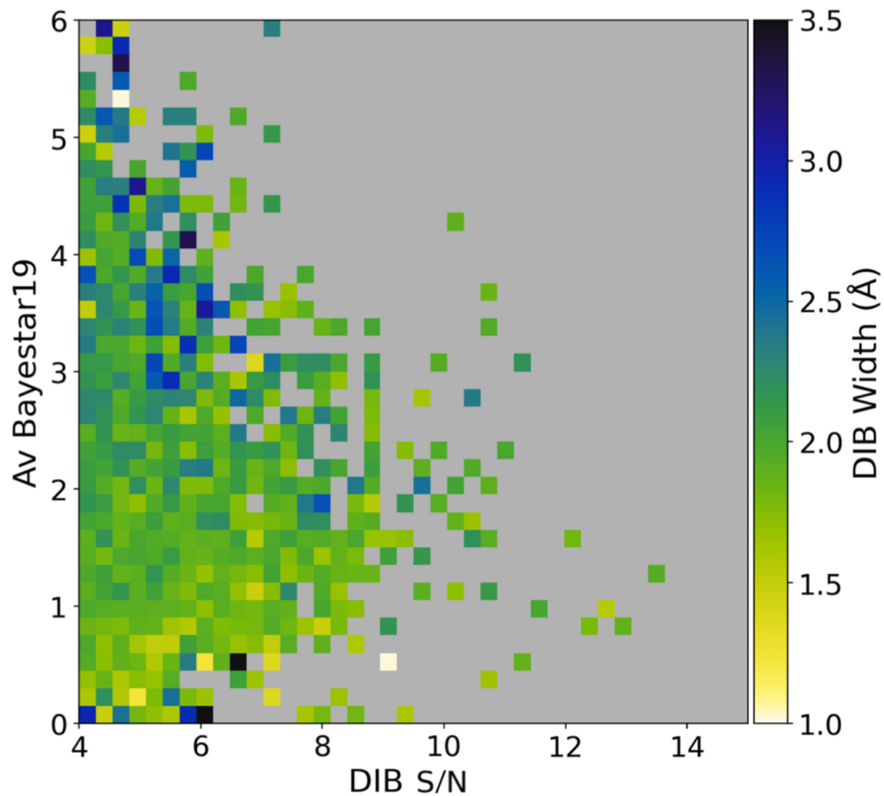
Figure 9. from Andrew K. Saydjari et al 2023 Astrophys. J. 954 doi:10.3847/1538-4357/acd454 https://dx.doi.org/10.3847/1538-4357/acd454 © 2023. The Author(s). Published by the American Astronomical Society.
