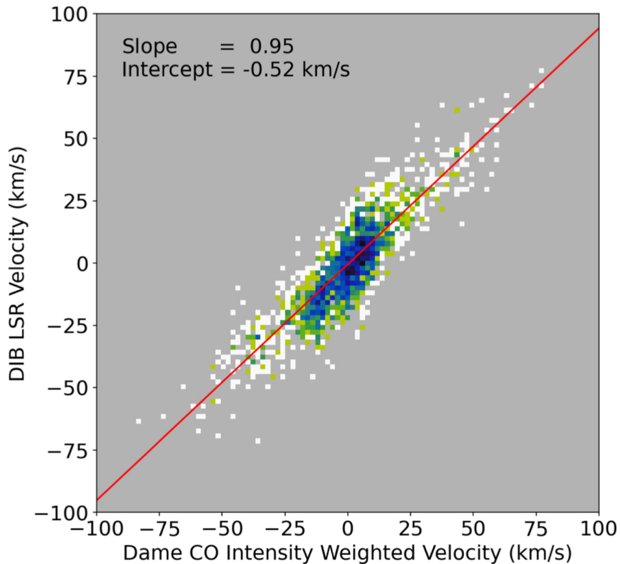
Figure 8. from Andrew K. Saydjari et al 2023 Astrophys. J. 954 doi:10.3847/1538-4357/acd454 https://dx.doi.org/10.3847/1538-4357/acd454 © 2023. The Author(s). Published by the American Astronomical Society.
