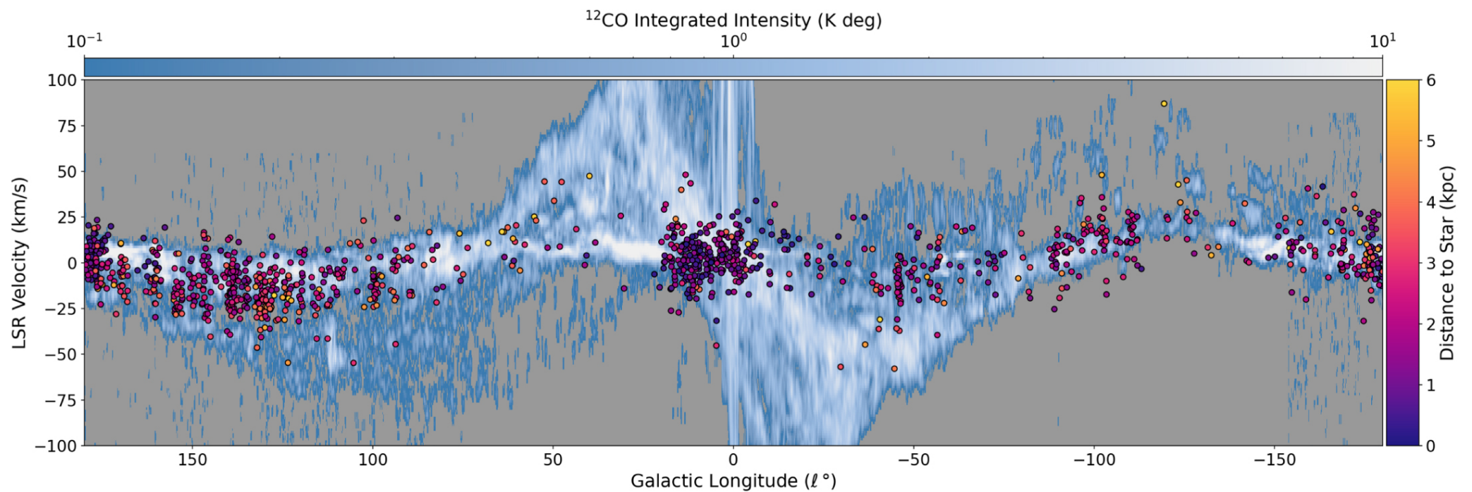
Figure 7. from Andrew K. Saydjari et al 2023 Astrophys. J. 954 doi:10.3847/1538-4357/acd454 https://dx.doi.org/10.3847/1538-4357/acd454 © 2023. The Author(s). Published by the American Astronomical Society.
