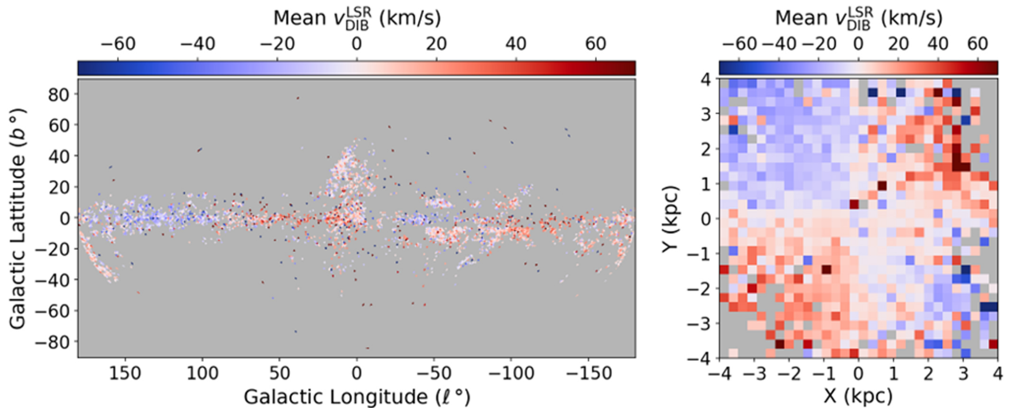
Figure 5. from Andrew K. Saydjari et al 2023 Astrophys. J. 954 doi:10.3847/1538-4357/acd454 https://dx.doi.org/10.3847/1538-4357/acd454 © 2023. The Author(s). Published by the American Astronomical Society.
