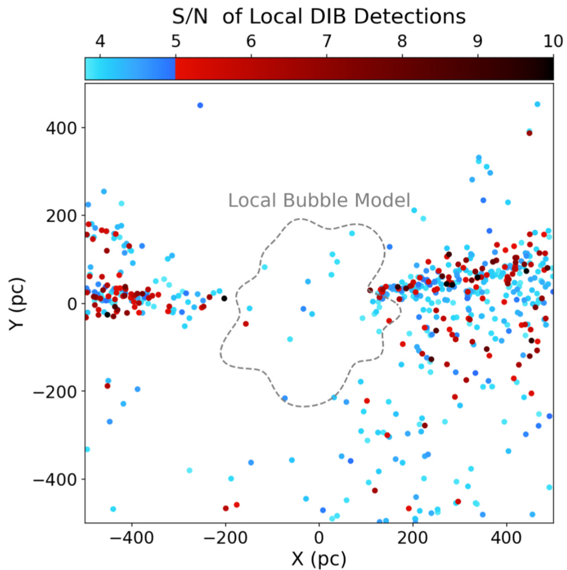
Figure 2. from Andrew K. Saydjari et al 2023 Astrophys. J. 954 doi:10.3847/1538-4357/acd454 https://dx.doi.org/10.3847/1538-4357/acd454 © 2023. The Author(s). Published by the American Astronomical Society.
