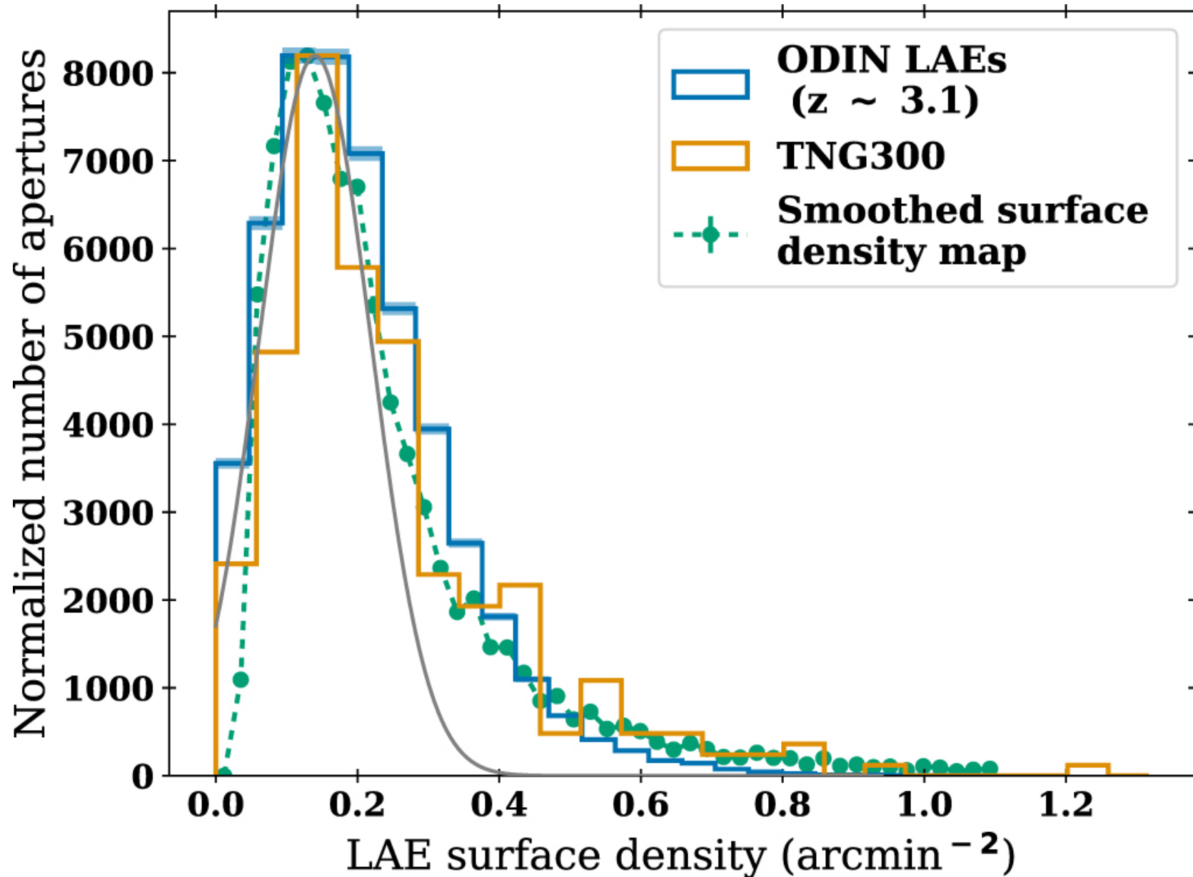
Figure 6. from Vandana Ramakrishnan et al 2023 Astrophys. J. 951 doi:10.3847/1538-4357/acd341 https://dx.doi.org/10.3847/1538-4357/acd341 © 2023. The Author(s). Published by the American Astronomical Society.
