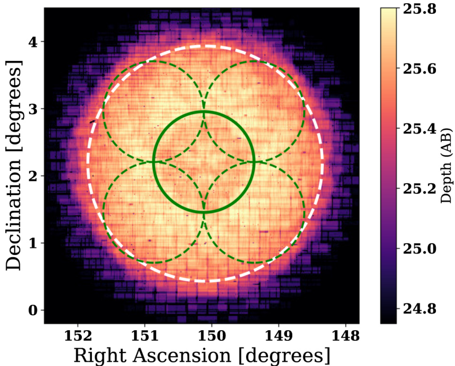
Figure 1. from Vandana Ramakrishnan et al 2023 Astrophys. J. 951 doi:10.3847/1538-4357/acd341 https://dx.doi.org/10.3847/1538-4357/acd341 © 2023. The Author(s). Published by the American Astronomical Society.
