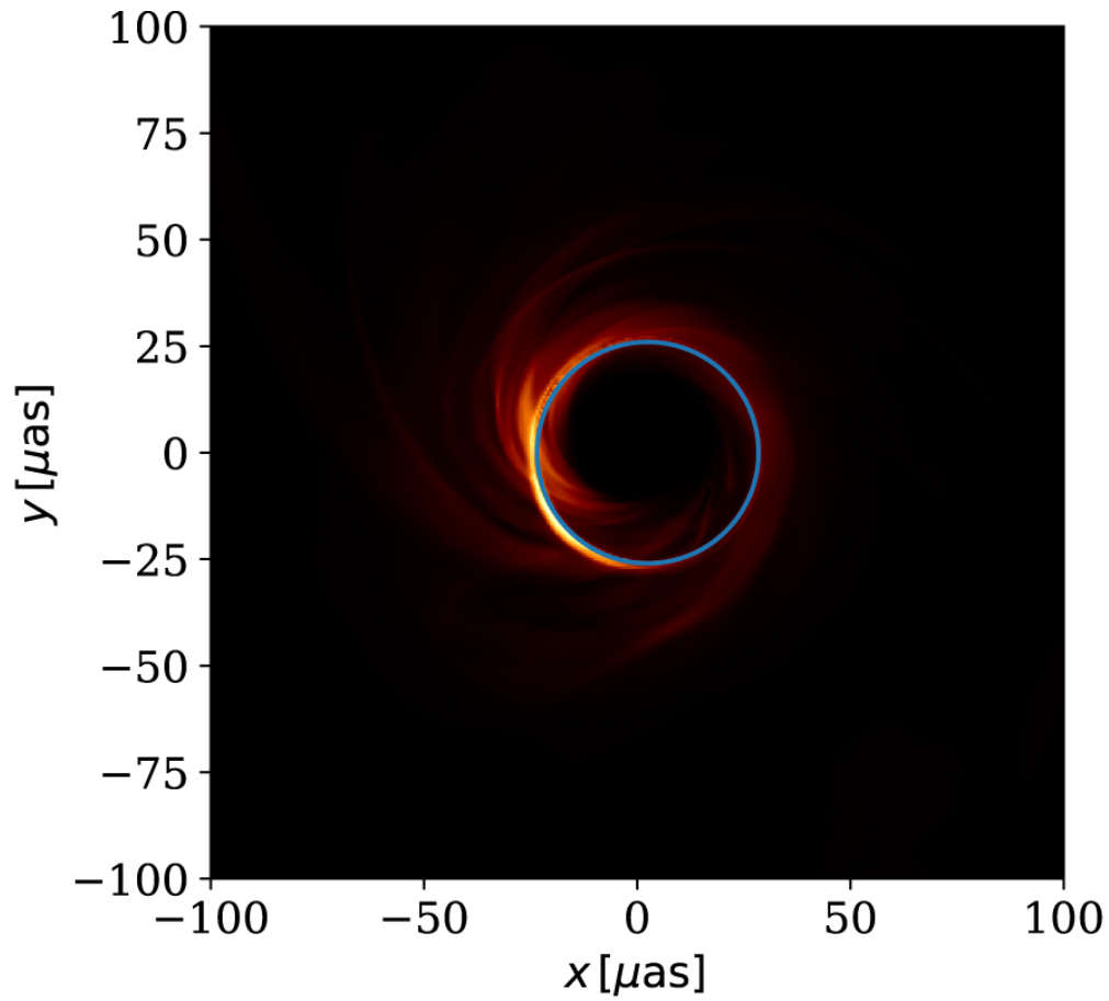
Figure 2. from Nicholas S. Conroy et al 2023 Astrophys. J. 951 doi:10.3847/1538-4357/acd2c8 https://dx.doi.org/10.3847/1538-4357/acd2c8 © 2023. The Author(s). Published by the American Astronomical Society.
