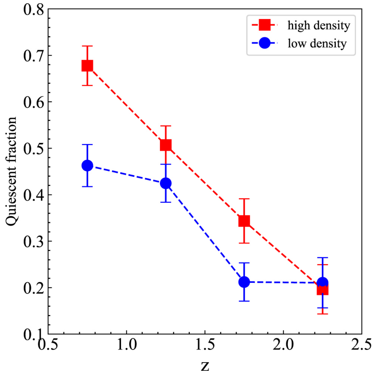
Figure 8. from Jie Song et al 2023 Astrophys. J. 950 doi:10.3847/1538-4357/acd174 https://dx.doi.org/10.3847/1538-4357/acd174 © 2023. The Author(s). Published by the American Astronomical Society.
