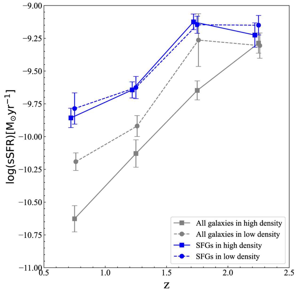
Figure 7. from Jie Song et al 2023 Astrophys. J. 950 doi:10.3847/1538-4357/acd174 https://dx.doi.org/10.3847/1538-4357/acd174 © 2023. The Author(s). Published by the American Astronomical Society.
