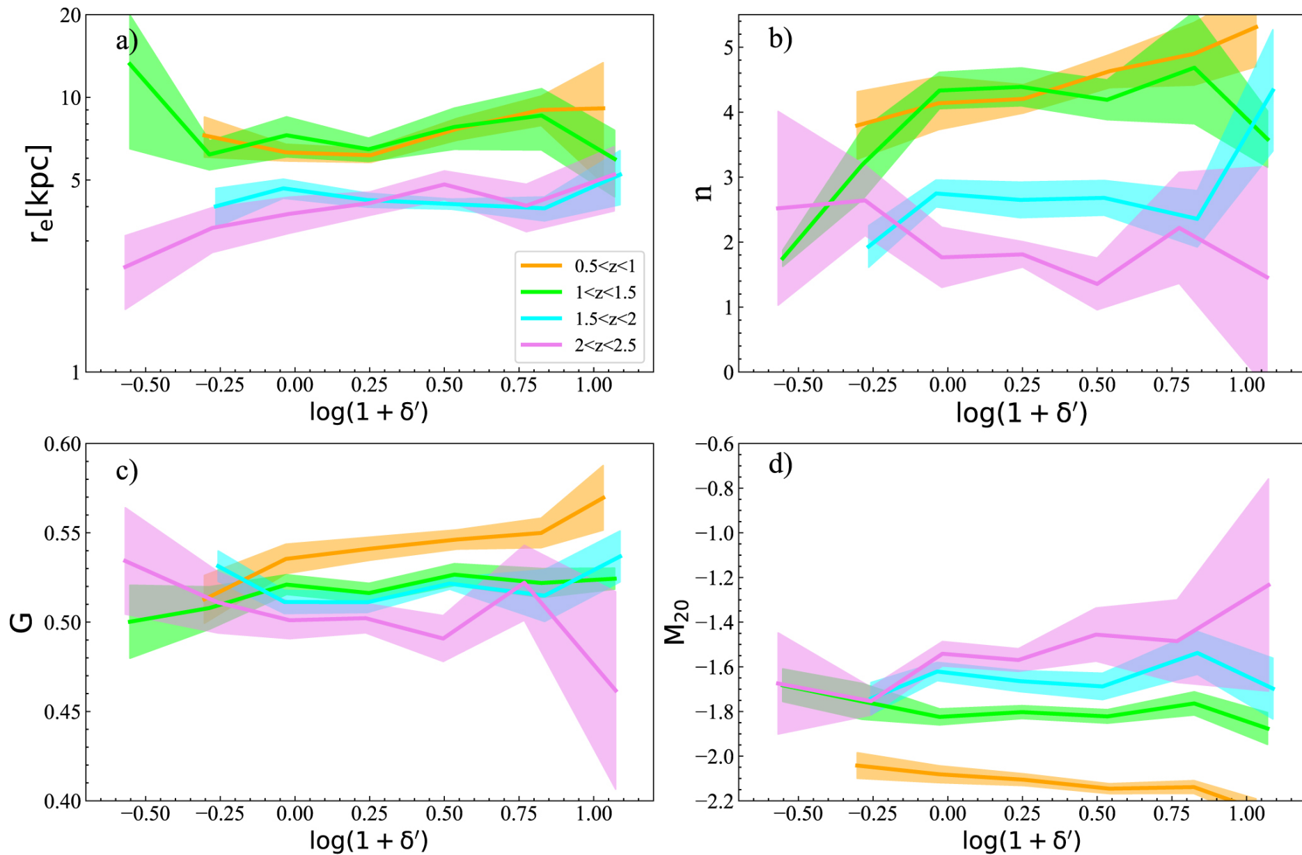
Figure 6. from Jie Song et al 2023 Astrophys. J. 950 doi:10.3847/1538-4357/acd174 https://dx.doi.org/10.3847/1538-4357/acd174 © 2023. The Author(s). Published by the American Astronomical Society.
