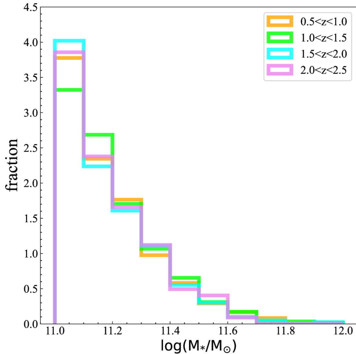
Figure 3. from Jie Song et al 2023 Astrophys. J. 950 doi:10.3847/1538-4357/acd174 https://dx.doi.org/10.3847/1538-4357/acd174 © 2023. The Author(s). Published by the American Astronomical Society.
