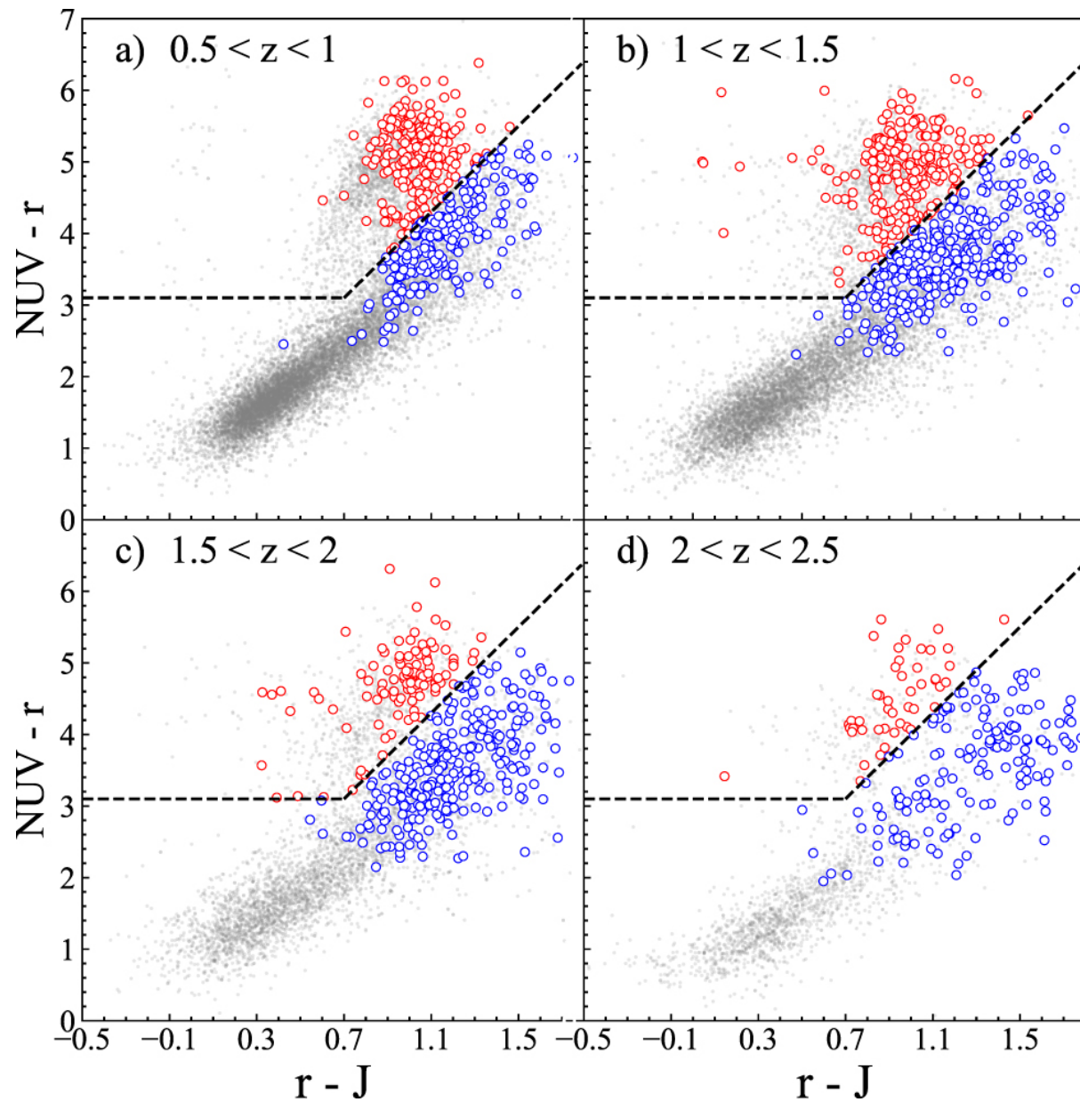
Figure 1. from Jie Song et al 2023 Astrophys. J. 950 doi:10.3847/1538-4357/acd174 https://dx.doi.org/10.3847/1538-4357/acd174 © 2023. The Author(s). Published by the American Astronomical Society.
