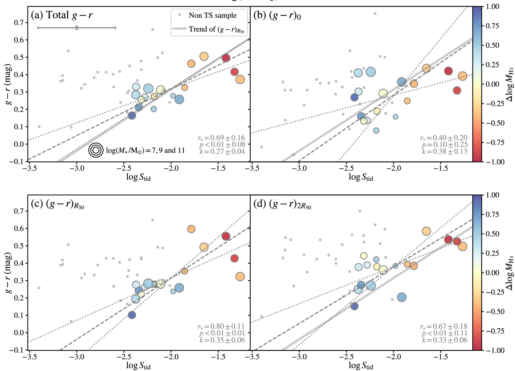
Figure 7. from Xuchen Lin et al 2023 Astrophys. J. 956 doi:10.3847/1538-4357/accea2 https://dx.doi.org/10.3847/1538-4357/accea2 © 2023. The Author(s). Published by the American Astronomical Society.
