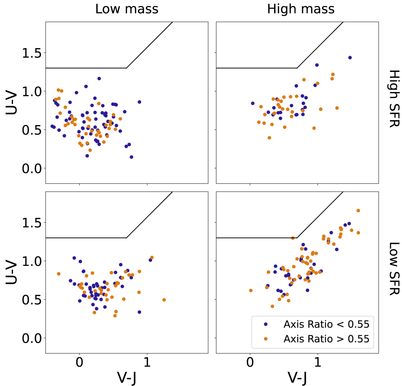
Figure 8. from Brian Lorenz et al 2023 Astrophys. J. 951 doi:10.3847/1538-4357/acdd1 https://dx.doi.org/10.3847/1538-4357/acdd1 © 2023. The Author(s). Published by the American Astronomical Society.
