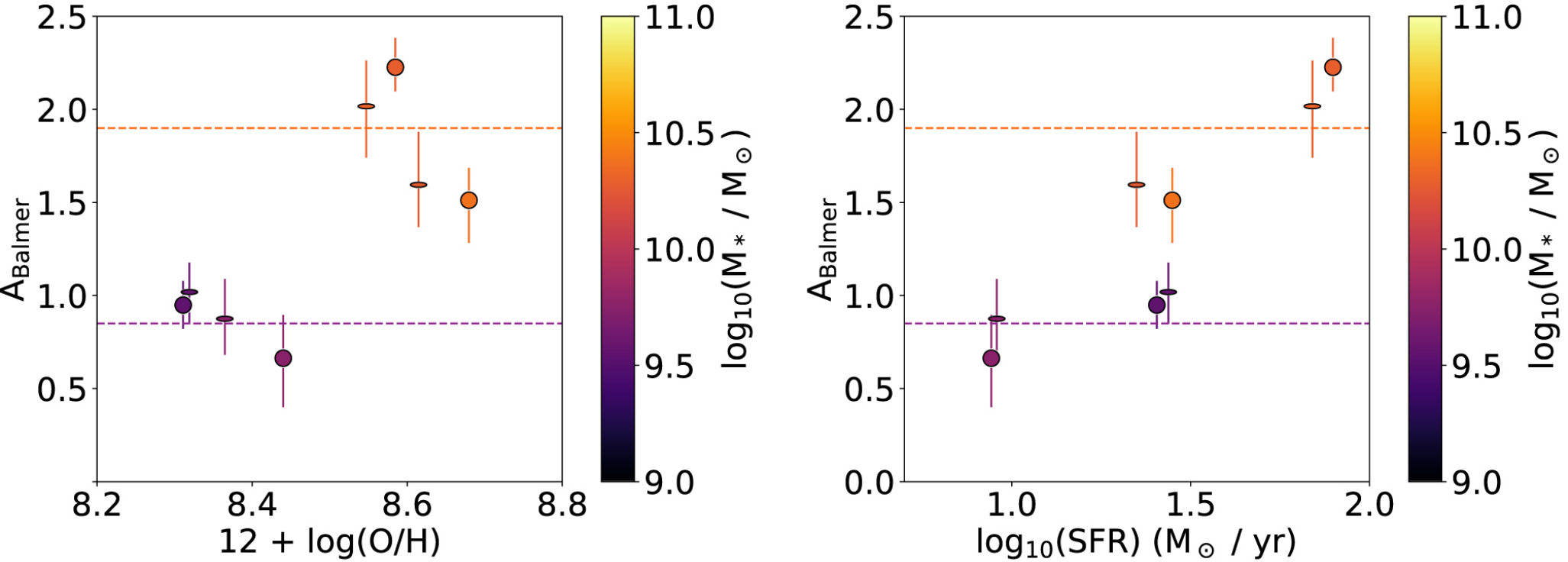
Figure 11. from Brian Lorenz et al 2023 Astrophys. J. 951 doi:10.3847/1538-4357/acdd1 https://dx.doi.org/10.3847/1538-4357/acdd1 © 2023. The Author(s). Published by the American Astronomical Society.
