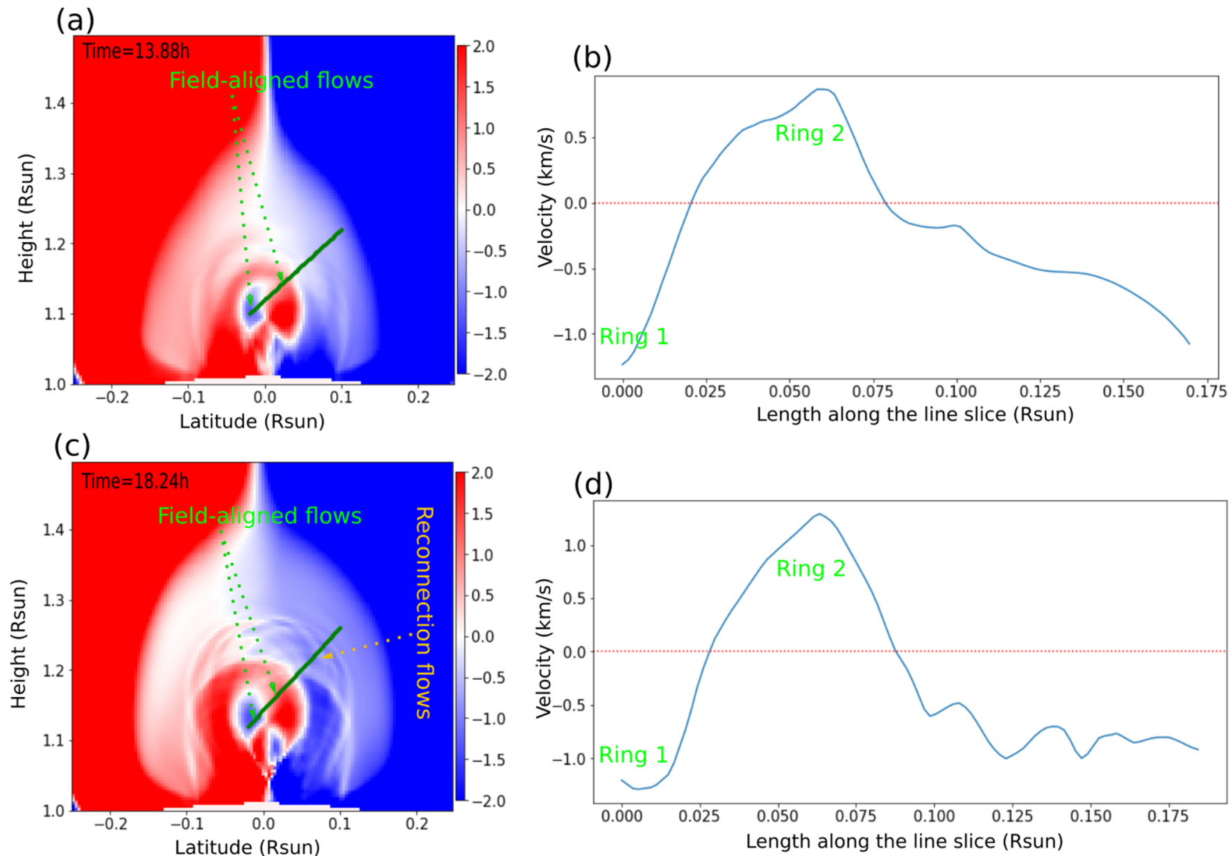
Figure 7. from Tie Liu et al 2023 Astrophys. J. 949 doi:10.3847/1538-4357/acca82 https://dx.doi.org/10.3847/1538-4357/acca82 © 2023. The Author(s). Published by the American Astronomical Society.
