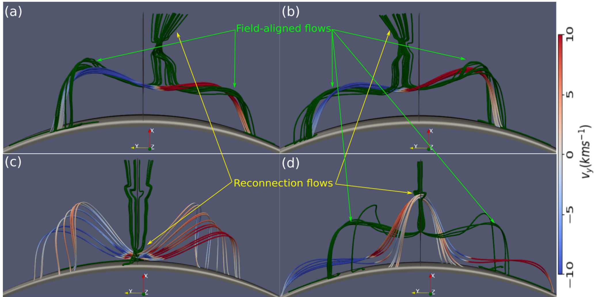
Figure 5. from Tie Liu et al 2023 Astrophys. J. 949 doi:10.3847/1538-4357/acca82 https://dx.doi.org/10.3847/1538-4357/acca82 © 2023. The Author(s). Published by the American Astronomical Society.
