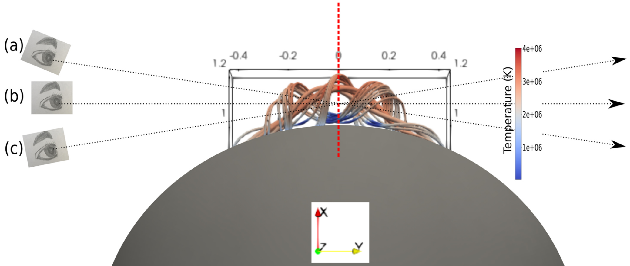
Figure 1. from Tie Liu et al 2023 Astrophys. J. 949 doi:10.3847/1538-4357/acca82 https://dx.doi.org/10.3847/1538-4357/acca82 © 2023. The Author(s). Published by the American Astronomical Society.
