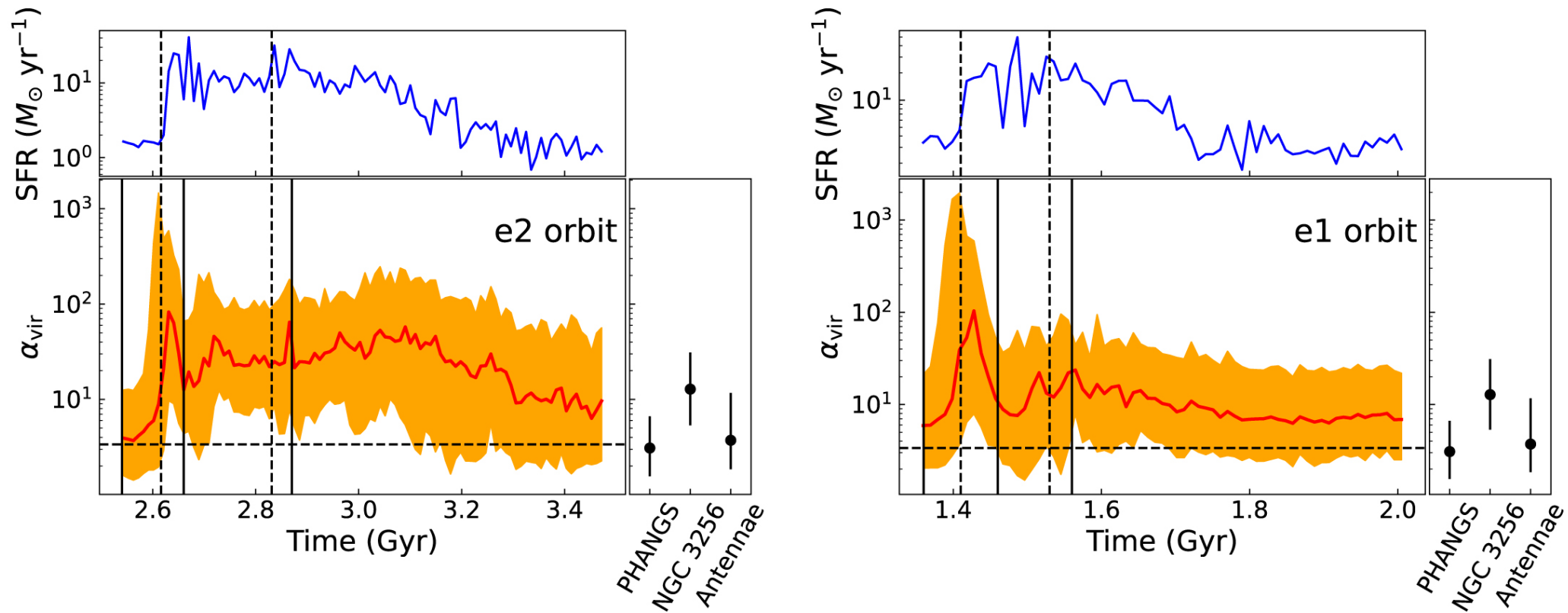
Figure 4. from Hao He et al 2023 Astrophys. J. 950 doi:10.3847/1538-4357/acca76 https://dx.doi.org/10.3847/1538-4357/acca76 © 2023. The Author(s). Published by the American Astronomical Society.
