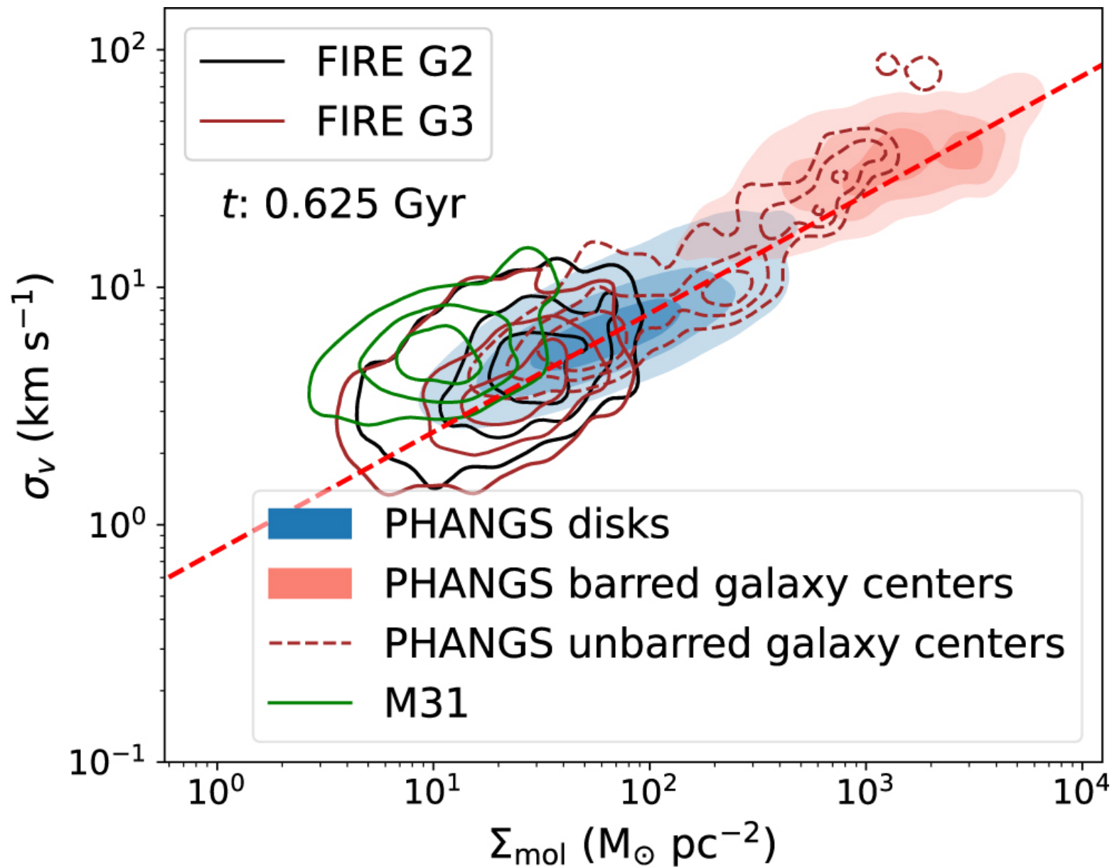
Figure 1. from Hao He et al 2023 Astrophys. J. 950 doi:10.3847/1538-4357/acca76 https://dx.doi.org/10.3847/1538-4357/acca76 © 2023. The Author(s). Published by the American Astronomical Society.
