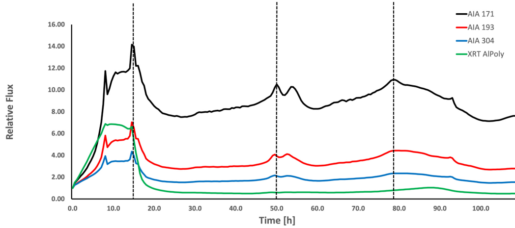
Figure 5. from Ofer Cohen et al 2023 Astrophys. J. 949 doi:10.3847/1538-4357/acc9c2 https://dx.doi.org/10.3847/1538-4357/acc9c2 © 2023. The Author(s). Published by the American Astronomical Society.
