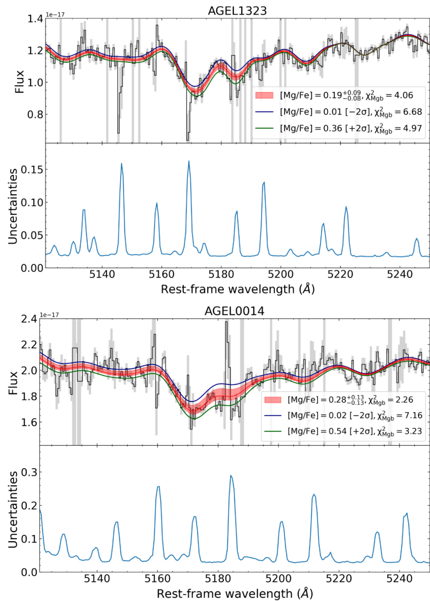
Figure 9. from Zhuyun Zhuang et al 2023 Astrophys. J. 948 doi:10.3847/1538-4357/acc79b https://dx.doi.org/10.3847/1538-4357/acc79b © 2023. The Author(s). Published by the American Astronomical Society.
