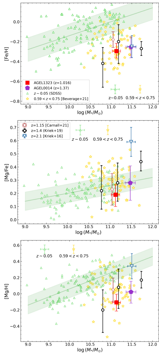
Figure 8. from Zhuyun Zhuang et al 2023 Astrophys. J. 948 doi:10.3847/1538-4357/acc79b https://dx.doi.org/10.3847/1538-4357/acc79b © 2023. The Author(s). Published by the American Astronomical Society.
