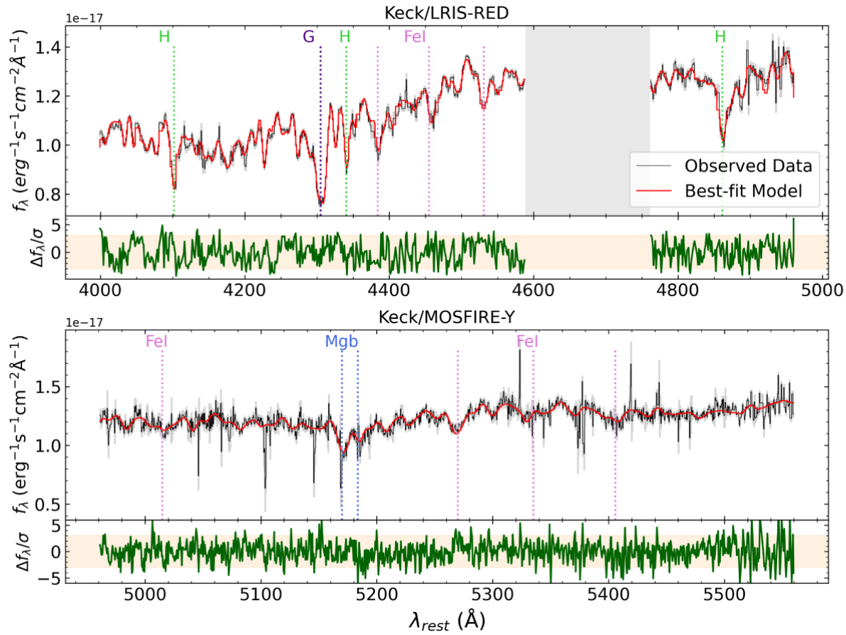
Figure 6. from Zhuyun Zhuang et al 2023 Astrophys. J. 948 doi:10.3847/1538-4357/acc79b https://dx.doi.org/10.3847/1538-4357/acc79b © 2023. The Author(s). Published by the American Astronomical Society.
