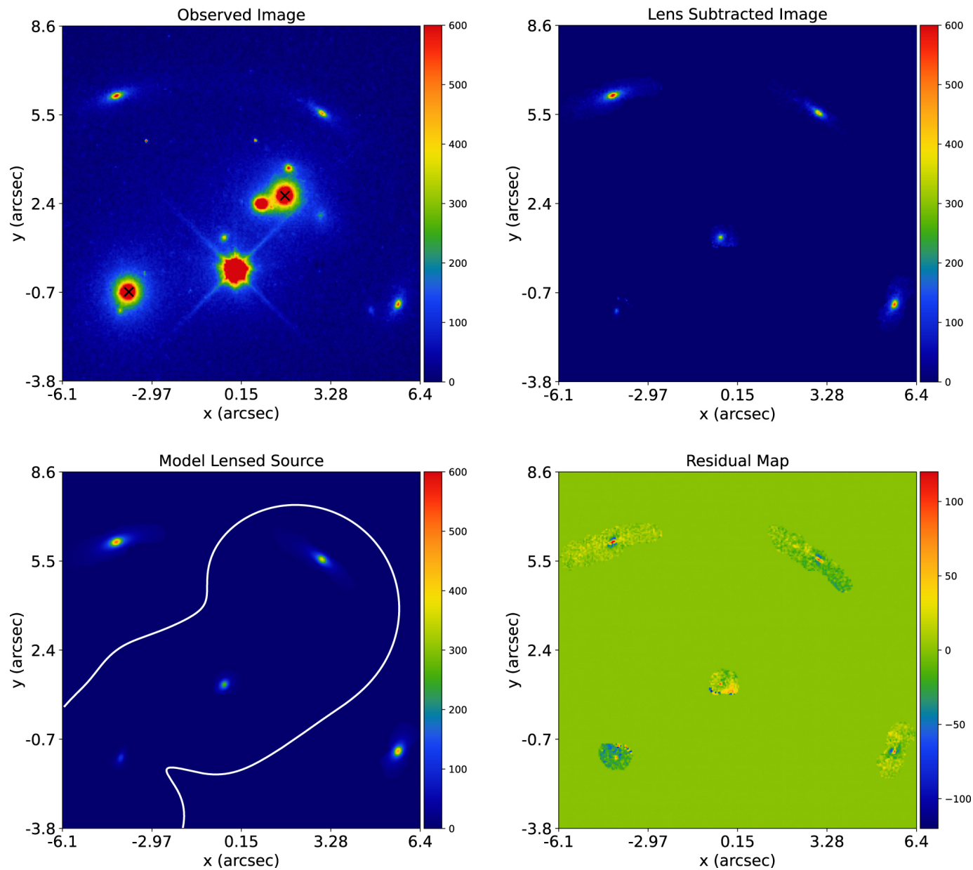
Figure 3. from Zhuyun Zhuang et al 2023 Astrophys. J. 948 doi:10.3847/1538-4357/acc79b https://dx.doi.org/10.3847/1538-4357/acc79b © 2023. The Author(s). Published by the American Astronomical Society.
