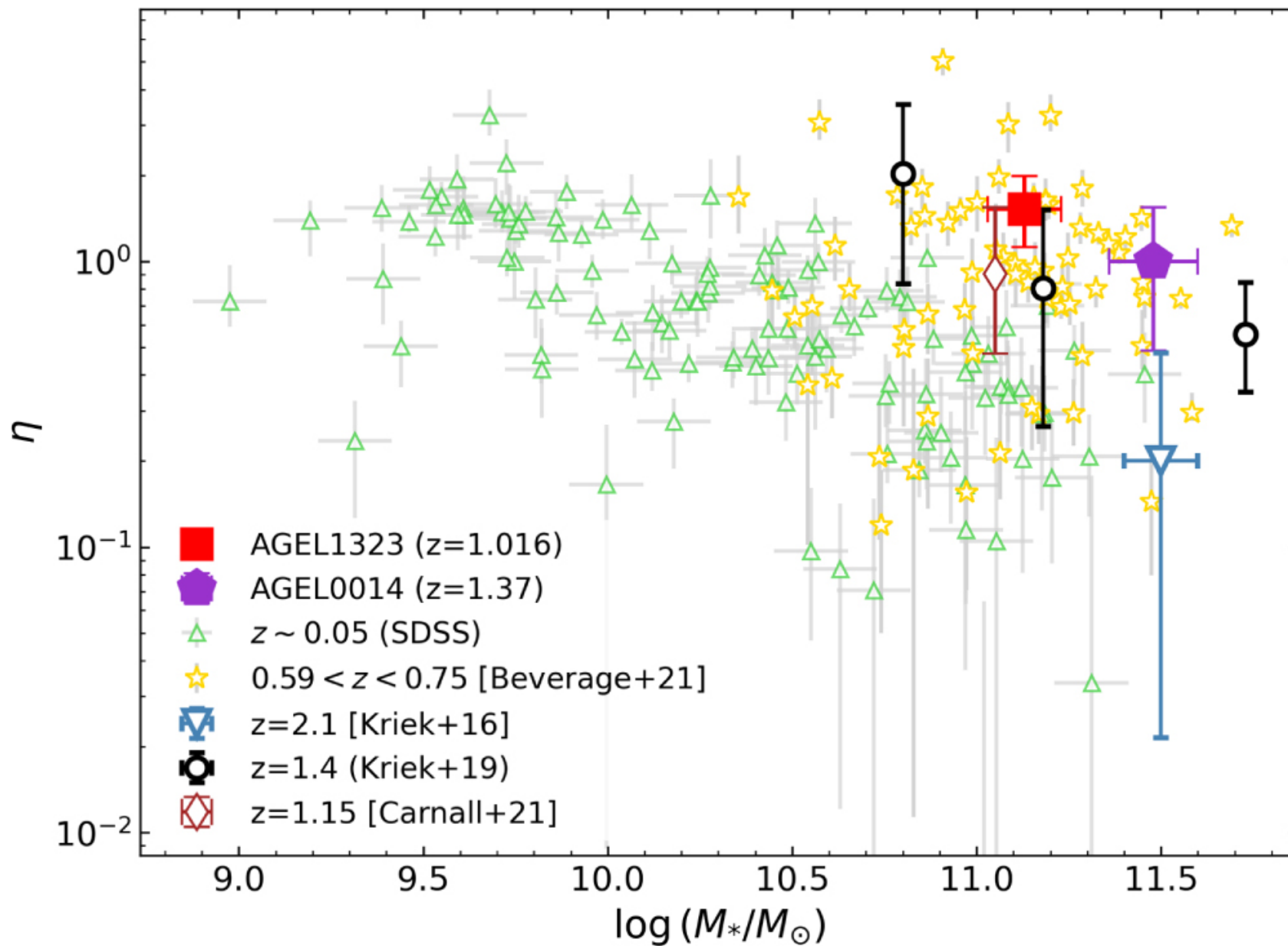
Figure 11. from Zhuyun Zhuang et al 2023 Astrophys. J. 948 doi:10.3847/1538-4357/acc79b https://dx.doi.org/10.3847/1538-4357/acc79b © 2023. The Author(s). Published by the American Astronomical Society.
