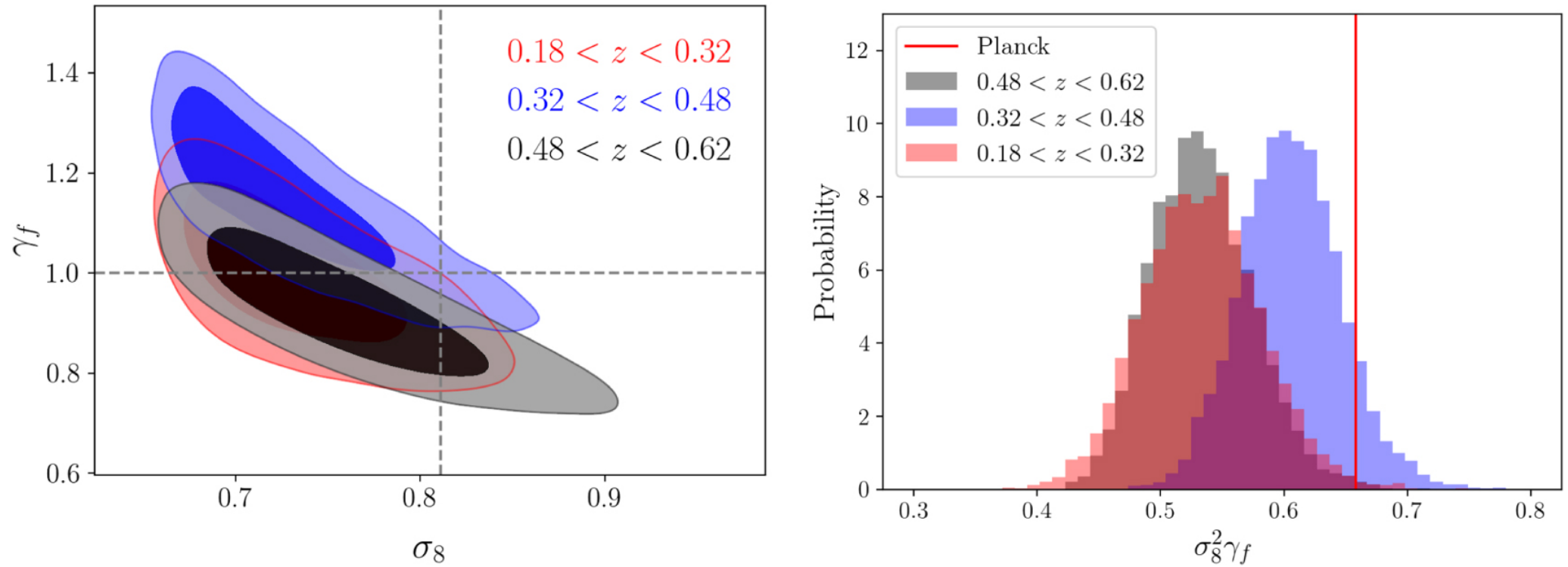
Figure 8. from Zhongxu Zhai et al 2023 Astrophys. J. 948 doi:10.3847/1538-4357/acc65b https://dx.doi.org/10.3847/1538-4357/acc65b © 2023. The Author(s). Published by the American Astronomical Society.
