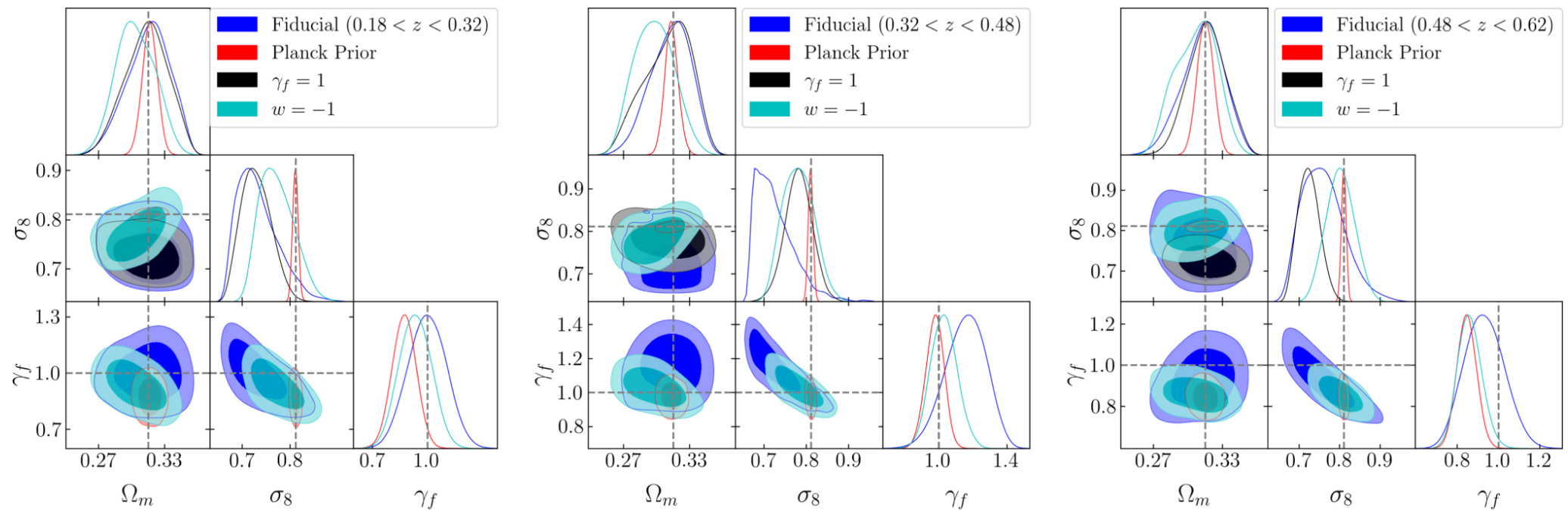
Figure 4. from Zhongxu Zhai et al 2023 Astrophys. J. 948 doi:10.3847/1538-4357/acc65b https://dx.doi.org/10.3847/1538-4357/acc65b © 2023. The Author(s). Published by the American Astronomical Society.
