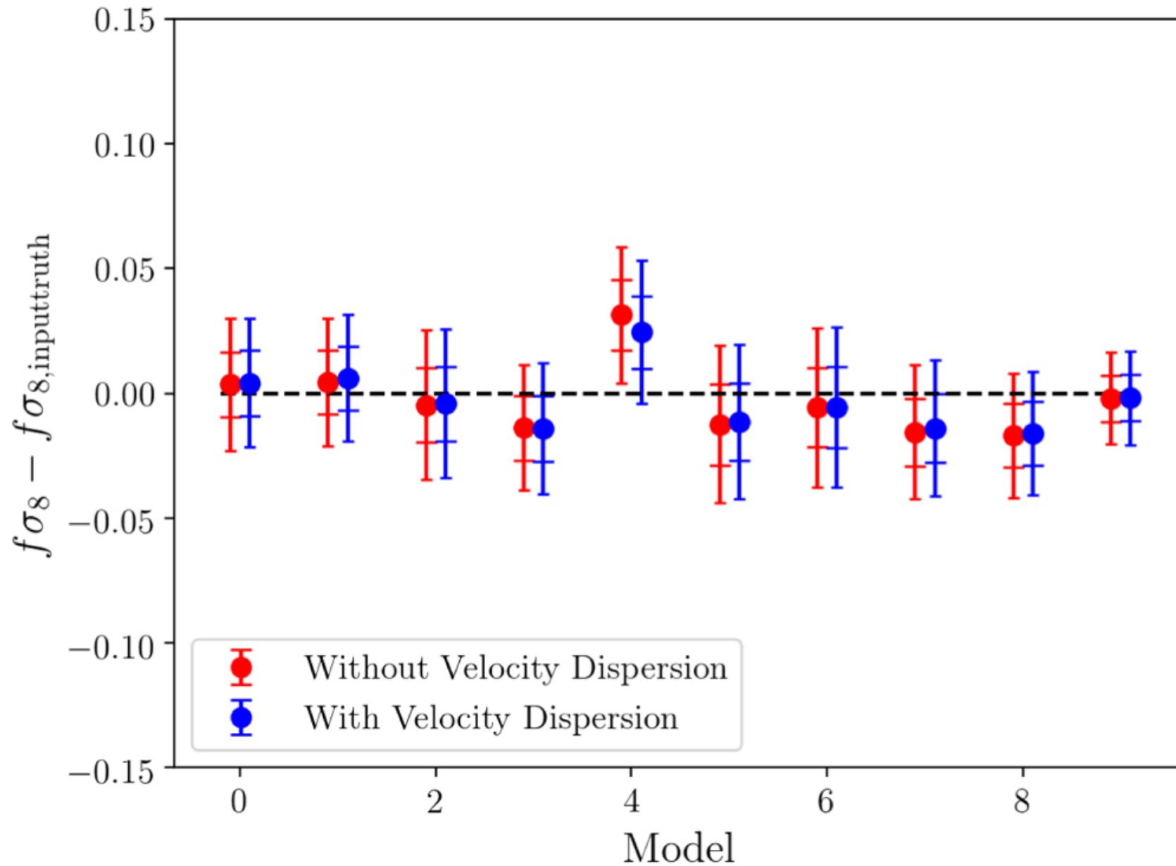
Figure 23. from Zhongxu Zhai et al 2023 Astrophys. J. 948 doi:10.3847/1538-4357/acc65b https://dx.doi.org/10.3847/1538-4357/acc65b © 2023. The Author(s). Published by the American Astronomical Society.
