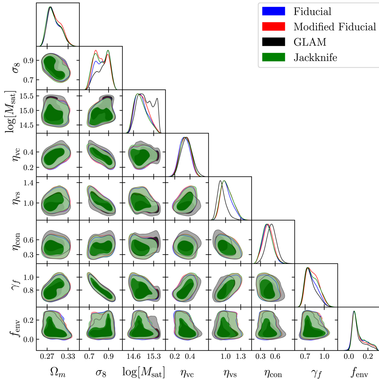
Figure 21. from Zhongxu Zhai et al 2023 Astrophys. J. 948 doi:10.3847/1538-4357/acc65b https://dx.doi.org/10.3847/1538-4357/acc65b © 2023. The Author(s). Published by the American Astronomical Society.
