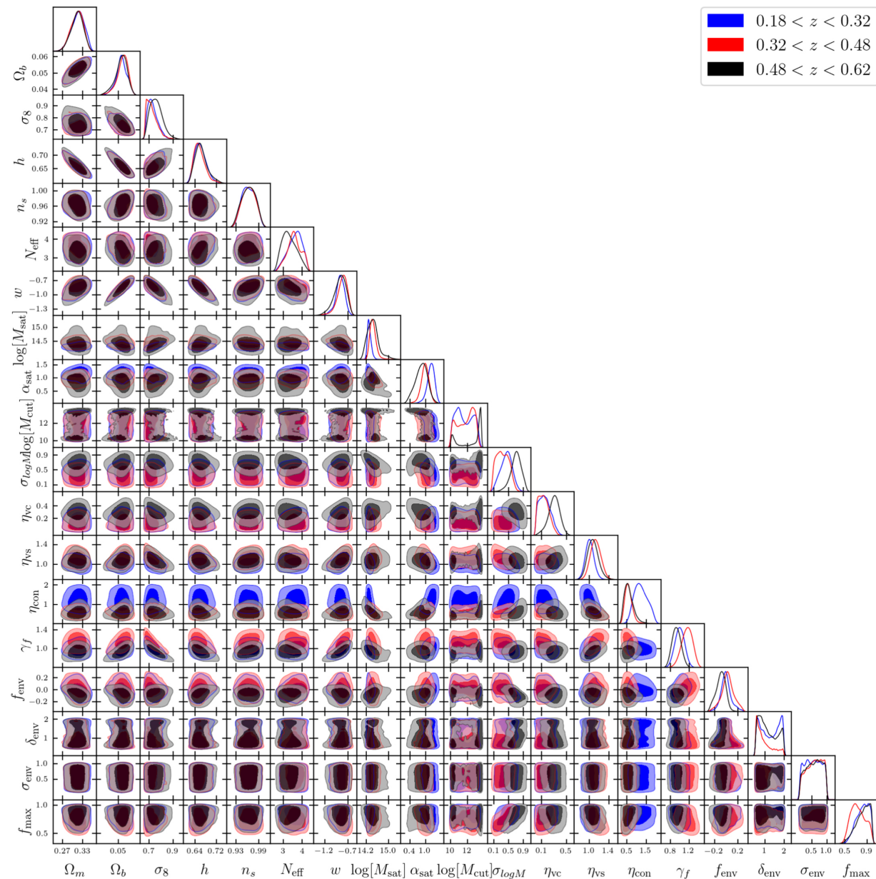
Figure 20. from Zhongxu Zhai et al 2023 Astrophys. J. 948 doi:10.3847/1538-4357/acc65b https://dx.doi.org/10.3847/1538-4357/acc65b © 2023. The Author(s). Published by the American Astronomical Society.
