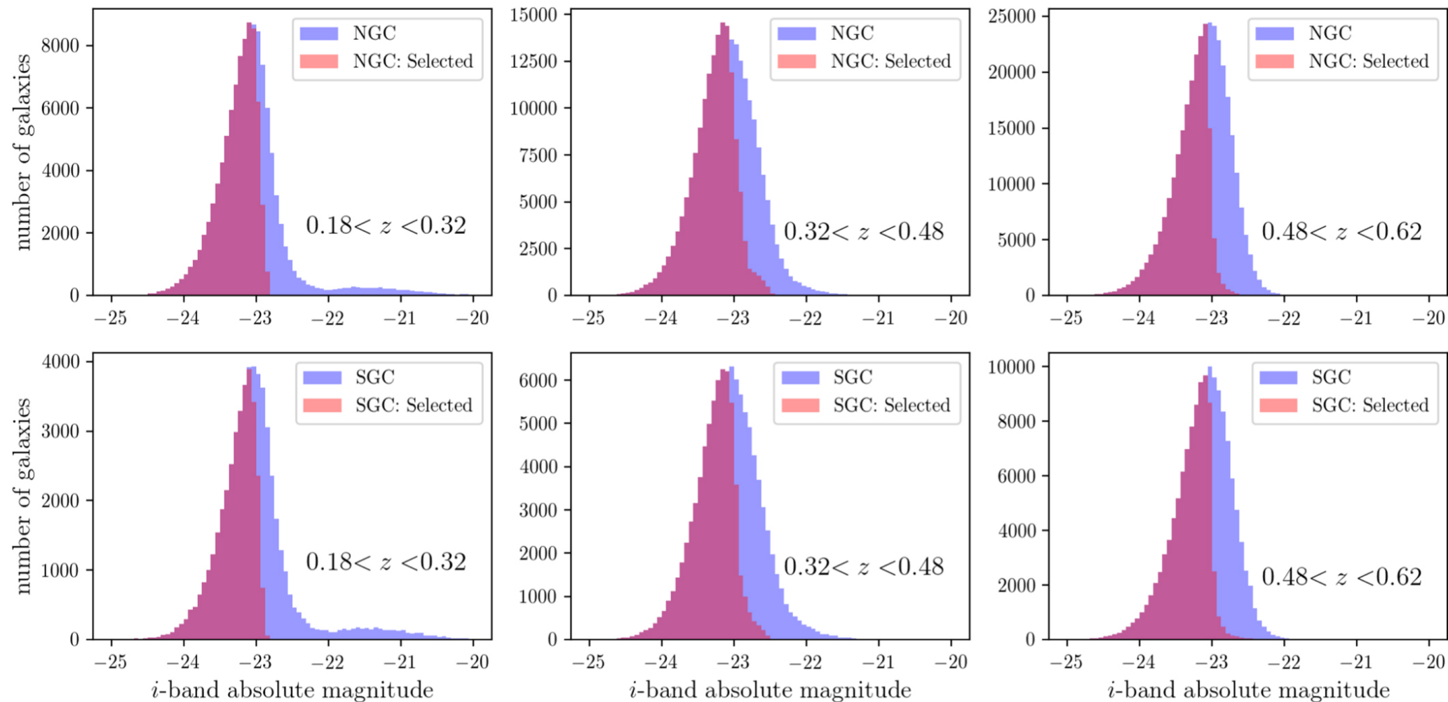
Figure 2. from Zhongxu Zhai et al 2023 Astrophys. J. 948 doi:10.3847/1538-4357/acc65b https://dx.doi.org/10.3847/1538-4357/acc65b © 2023. The Author(s). Published by the American Astronomical Society.
